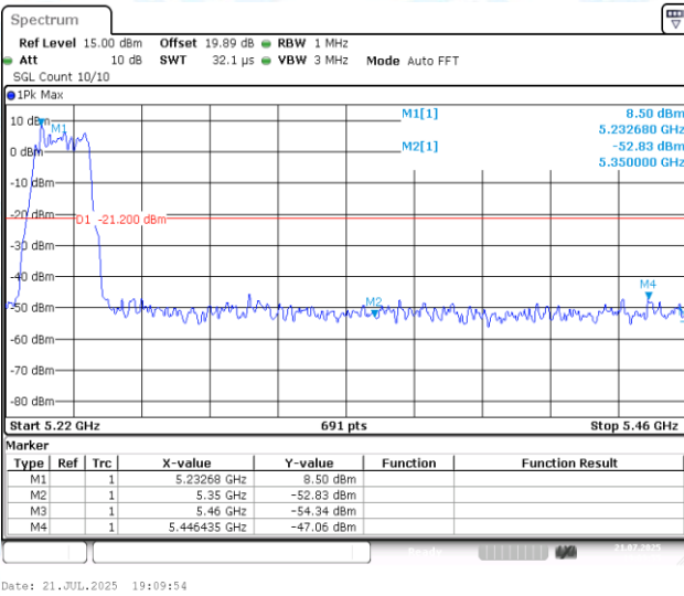
11AX20MIMO-Ant2-5240-PASS
