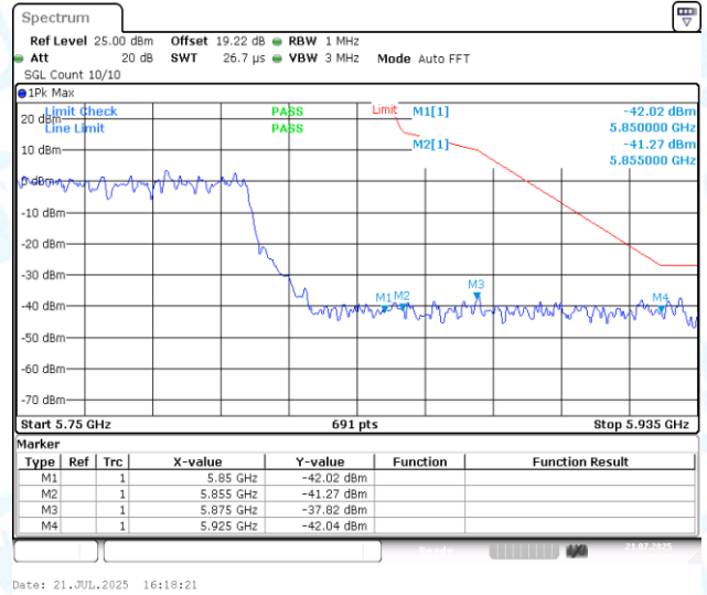
11AC80MIMO-Ant1-5775-PASS
