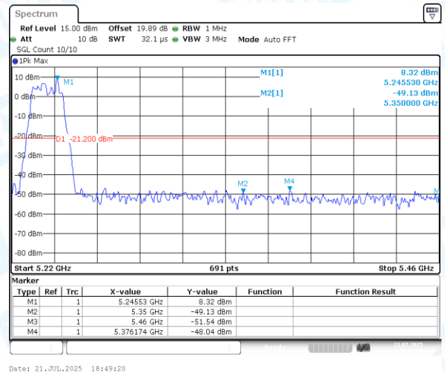
11AC20MIMO-Ant2-5240-PASS
