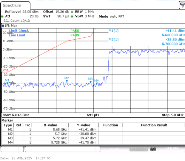
11AX80MIMO-Ant2-5775-PASS
