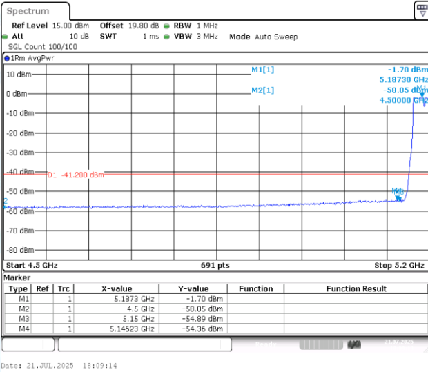
11N40MIMO-Ant2-5190-PASS
