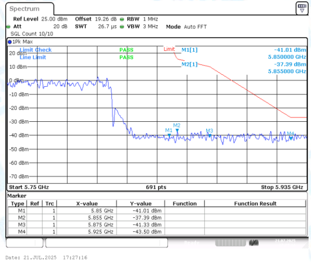
11AX80MIMO-Ant2-5775-PASS
