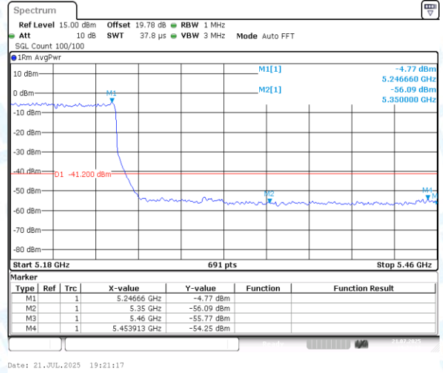
11AX80MIMO-Ant2-5210-PASS
