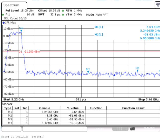
11AC20MIMO-Ant1-5240-PASS
