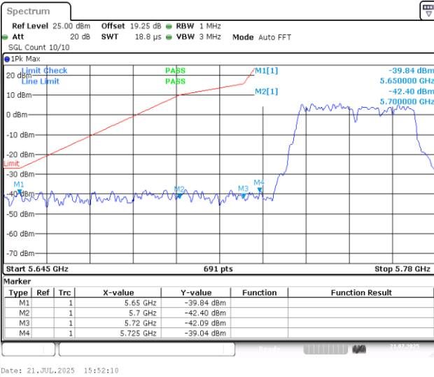
11AC40MIMO-Ant1-5755-PASS
