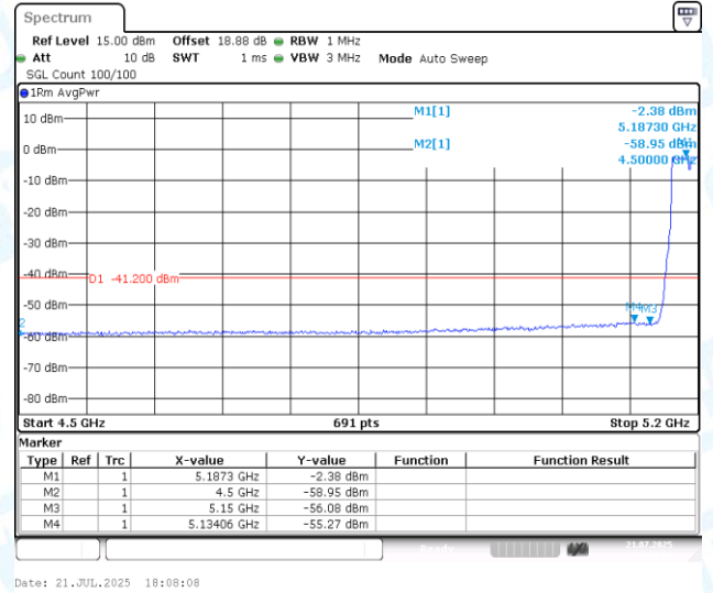
11N40MIMO-Ant1-5190-PASS
