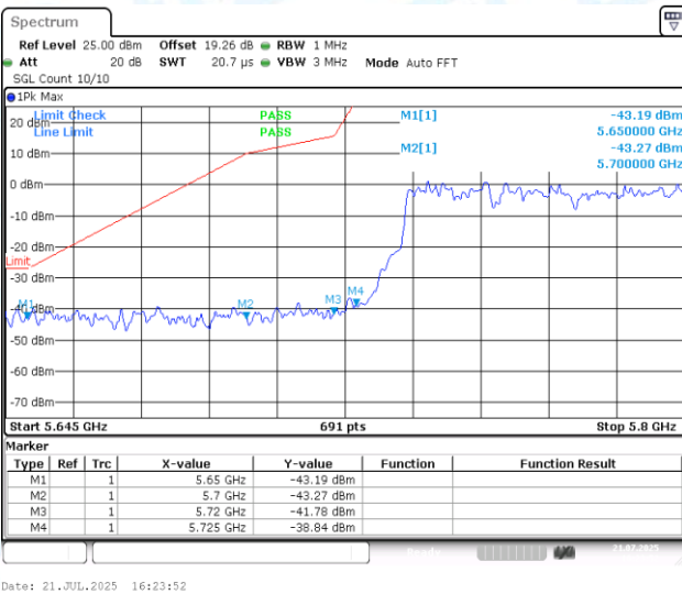
11AC80MIMO-Ant2-5775-PASS
