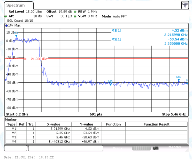
11N40MIMO-Ant2-5230-PASS
