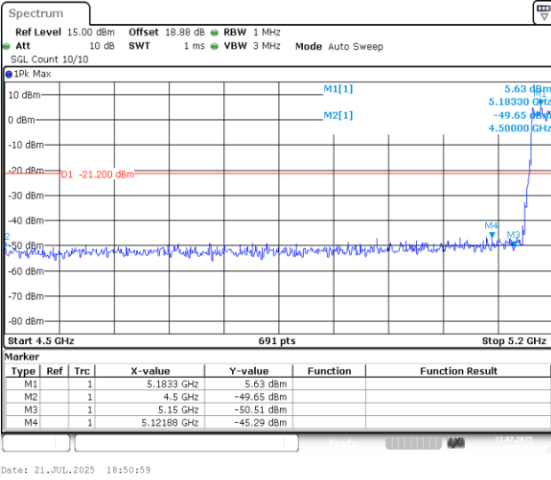
11AC40MIMO-Ant1-5190-PASS
