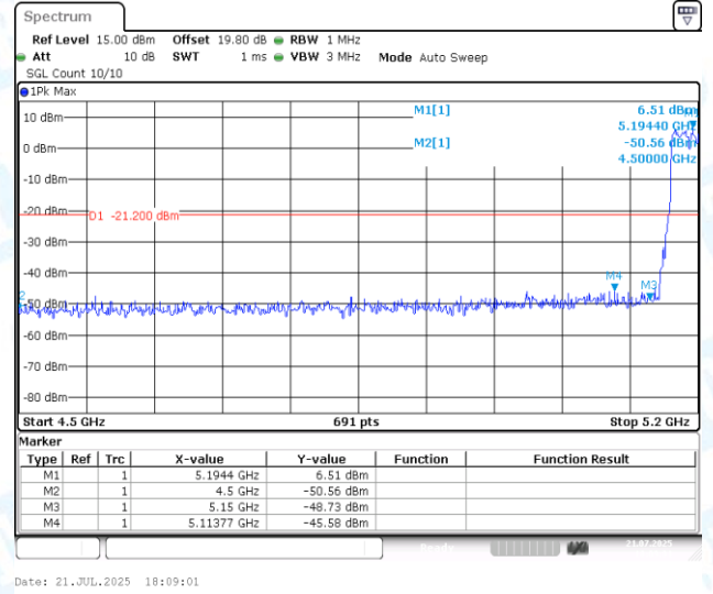
11N40MIMO-Ant2-5190-PASS
