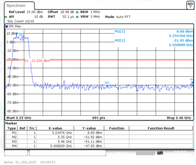
11AX20MIMO-Ant1-5240-PASS
