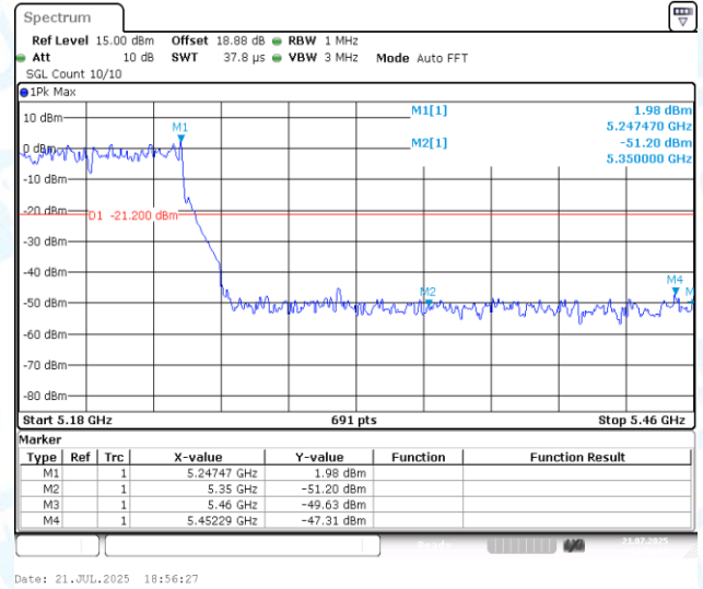
11AC80MIMO-Ant1-5210-PASS
