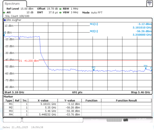
11AC80MIMO-Ant2-5210-PASS
