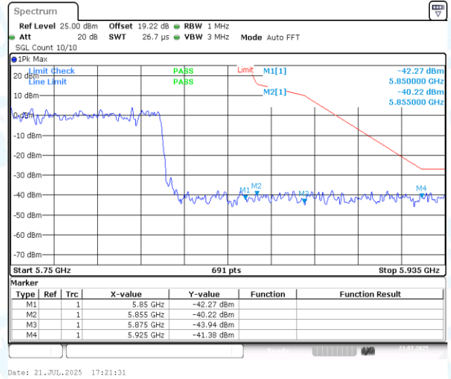
11AX80MIMO-Ant1-5775-PASS
