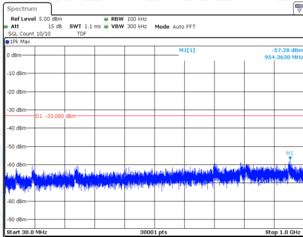
11G-CDD-Ant1-2412-0~Reference-PASS
