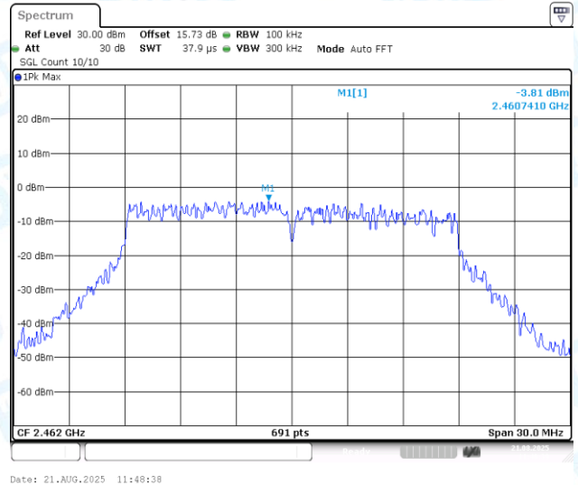
11N20MIMO-Ant2-2462-0~Reference-PASS
