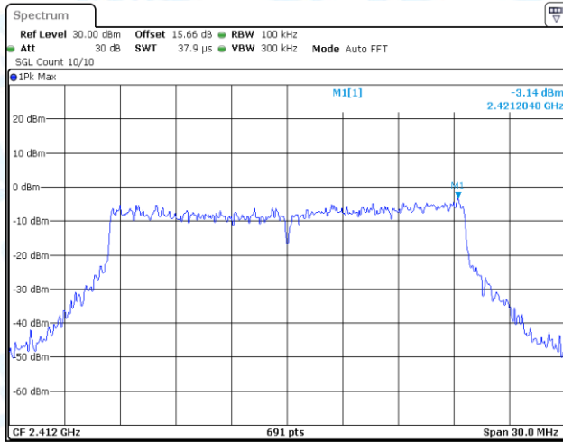
11AX20MIMO-Ant1-2412-0~Reference-PASS
