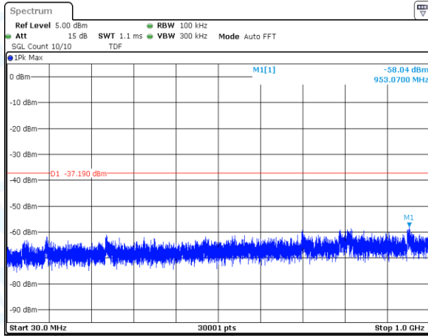
11N40MIMO-Ant1-2422-0~Reference-PASS
