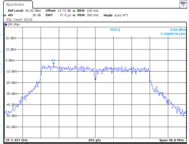
11N20MIMO-Ant2-2437-0~Reference-PASS
