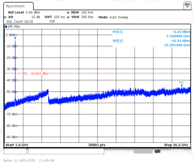
11N20MIMO-Ant2-2462-1000~26500-PASS
