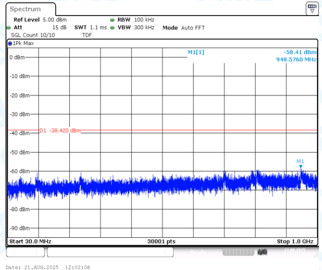
11N40MIMO-Ant2-2437-30~1000-PASS
