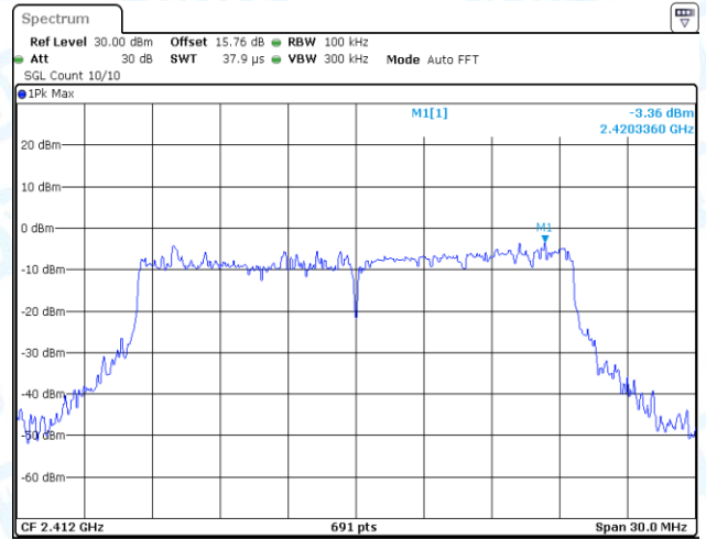
11AX20MIMO-Ant2-2412-0~Reference-PASS
