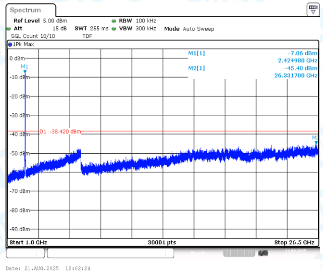
11N40MIMO-Ant2-2437-1000~26500-PASS
