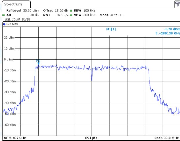
11AX20MIMO-Ant1-2437-0~Reference-PASS
