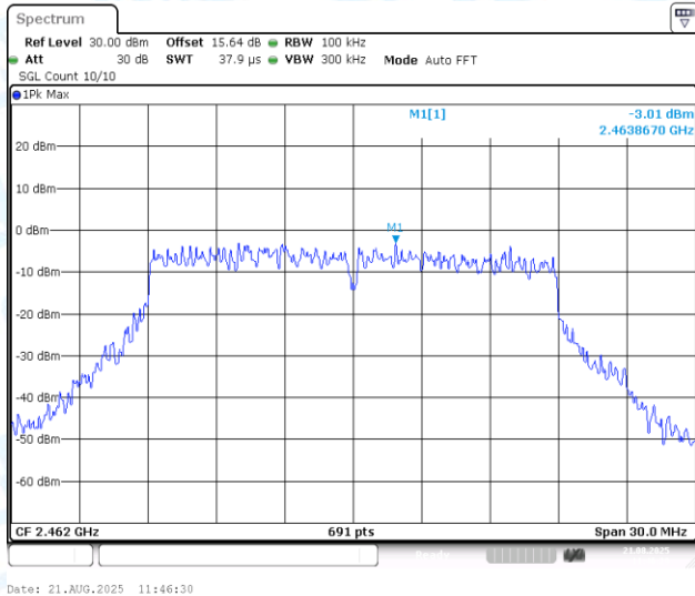
11N20MIMO-Ant1-2462-0~Reference-PASS
