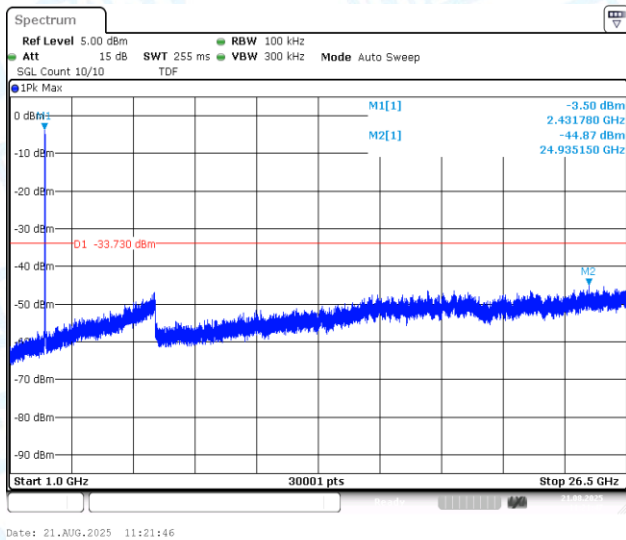
11G-CDD-Ant1-2437-1000~26500-PASS
