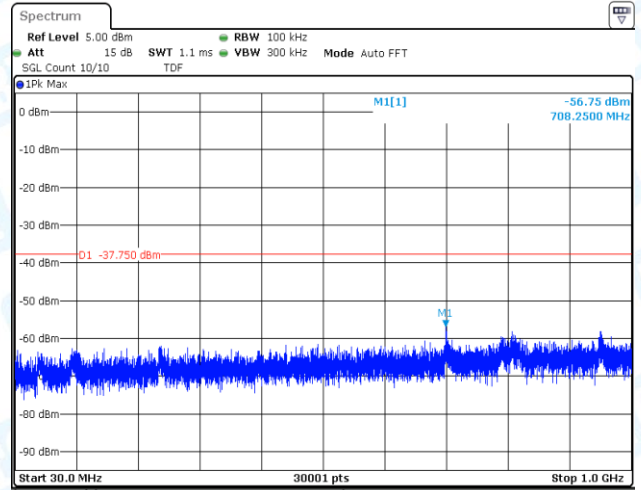
11N40MIMO-Ant2-2422-0~Reference-PASS
