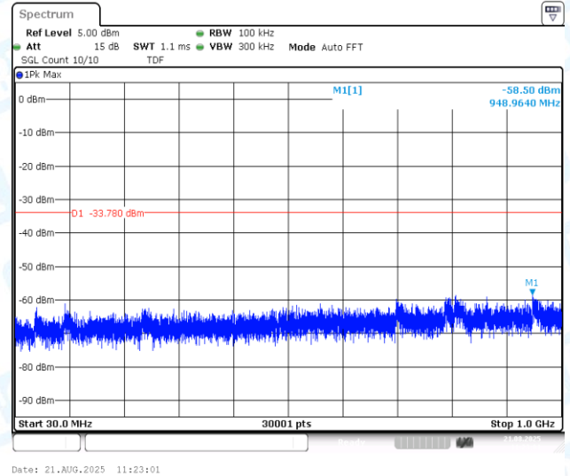
11G-CDD-Ant2-2437-30~1000-PASS
