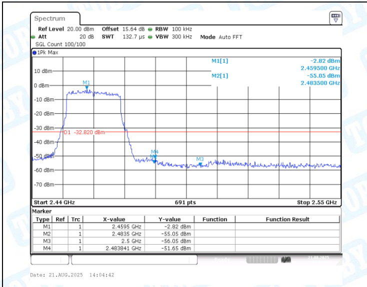
11AX20MIMO-Ant1-2462-PASS
