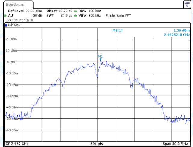
11B-CDD-Ant2-2462-0~Reference-PASS
