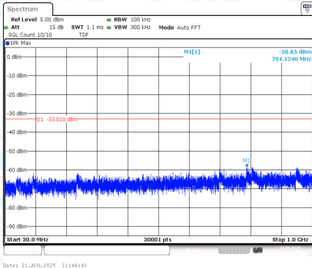
11N20MIMO-Ant1-2462-30~1000-PASS
