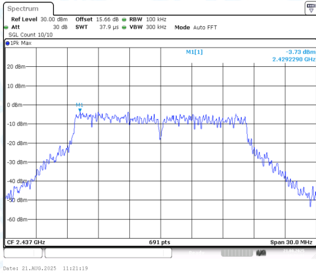
11G-CDD-Ant1-2437-0~Reference-PASS
