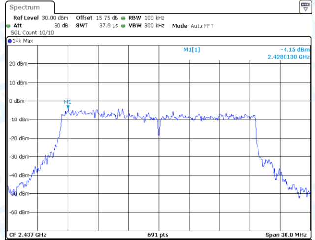
11AX20MIMO-Ant2-2437-0~Reference-PASS
