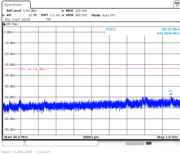
11G-CDD-Ant1-2437-30~1000-PASS
