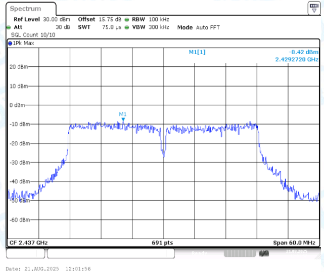
11N40MIMO-Ant2-2437-0~Reference-PASS
