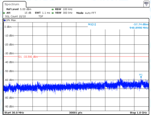
11G-CDD-Ant2-2412-0~Reference-PASS
