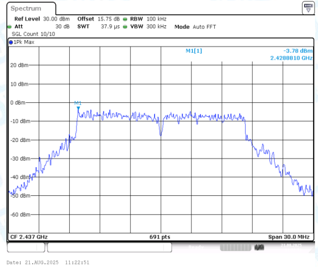
11G-CDD-Ant2-2437-0~Reference-PASS
