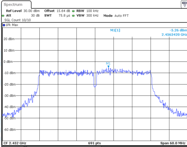
11N40MIMO-Ant1-2452-0~Reference-PASS
