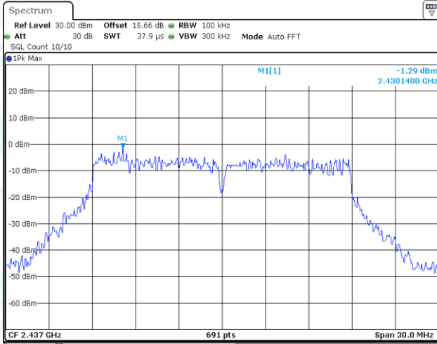
11N20MIMO-Ant1-2437-0~Reference-PASS
