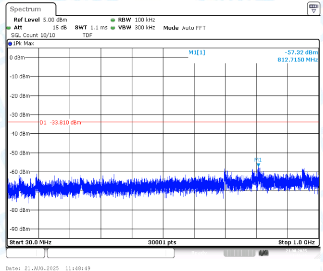
11N20MIMO-Ant2-2462-30~1000-PASS
