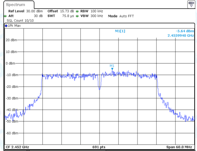
11N40MIMO-Ant2-2452-0~Reference-PASS
