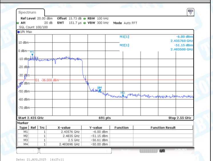
11AX40MIMO-Ant2-2452-PASS
