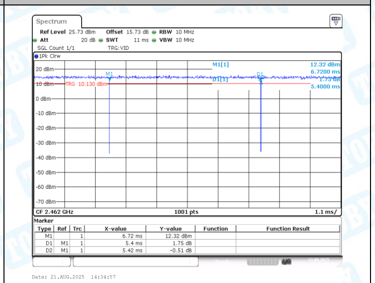
NTNV-11N20MIMO-Ant2-2462
