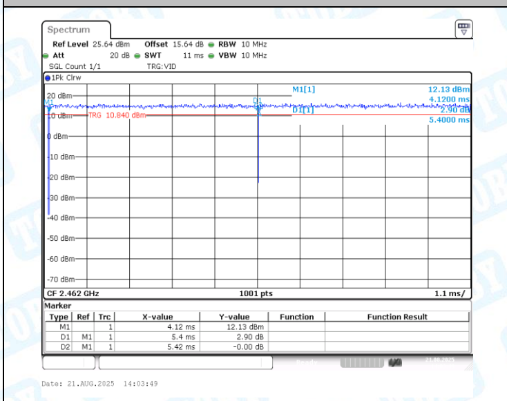
NTVN-11AX20MIMO-Ant1-2462
