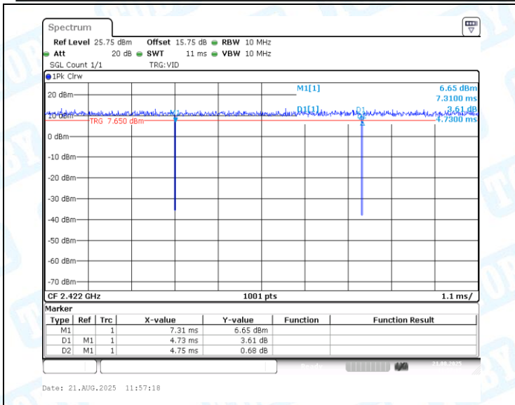
NTNV-11N40MIMO-Ant2-2422
