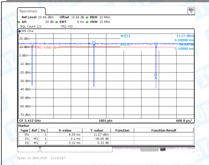
NTNV-11G-CDD-Ant1-2412
