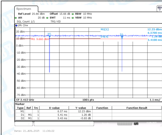
NTNV-11N20MIMO-Ant1-2412
