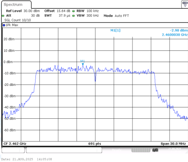
11AX20MIMO-Ant1-2462-0~Reference-PASS
