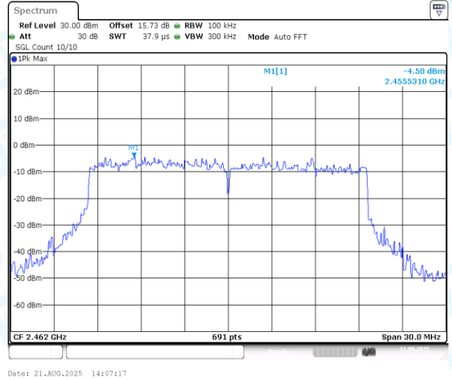
11AX20MIMO-Ant2-2462-0~Reference-PASS
