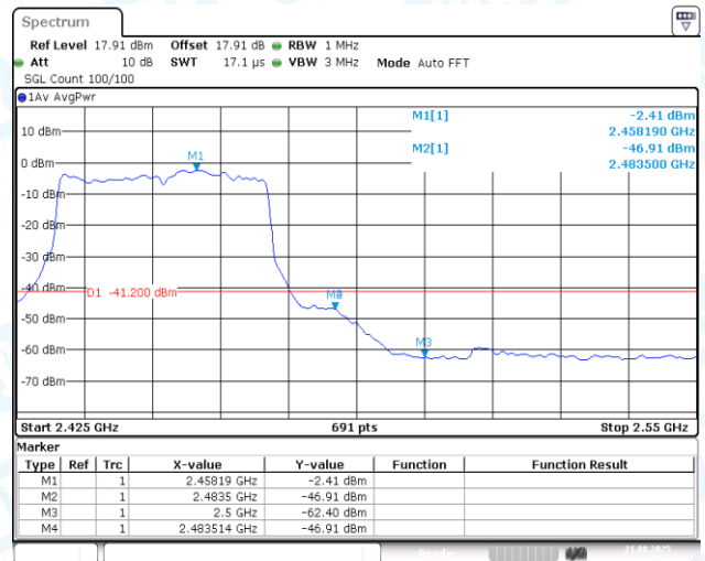
11AX40MIMO-Ant2-2452-PASS
