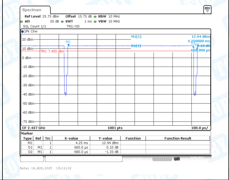
NTVN-11B-CDD-Ant2-2437
