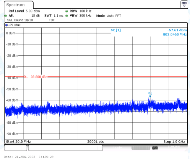
11AX40MIMO-Ant2-2437-30~1000-PASS
