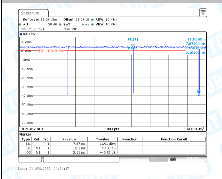
NTNV-11G-CDD-Ant1-2462
