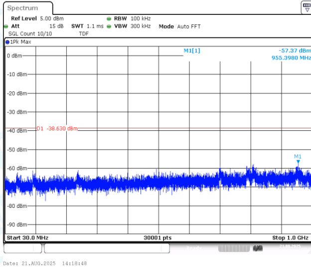
11AX40MIMO-Ant1-2437-30~1000-PASS
