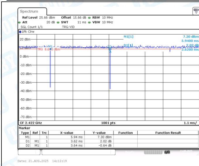
NTVN-11AX40MIMO-Ant1-2422
