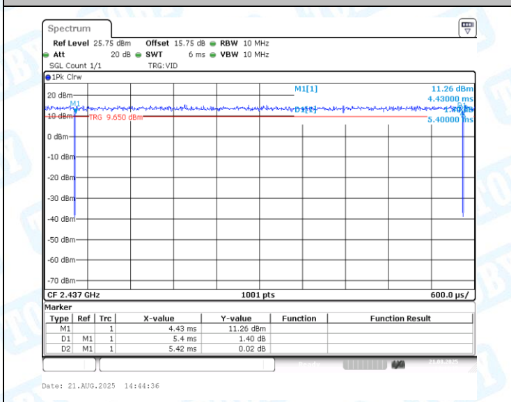
NTVN-11AX20MIMO-Ant2-2437
