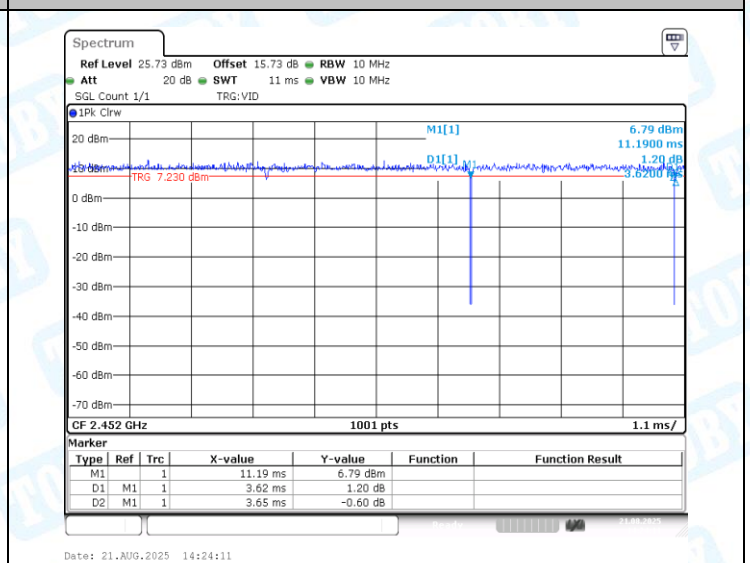
NTVN-11AX40MIMO-Ant2-2452
