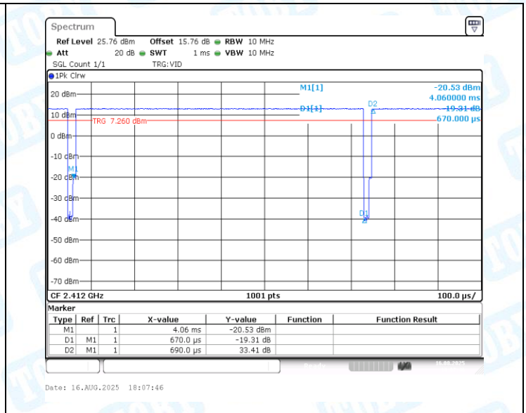
NTVN-11B-CDD-Ant2-2412
