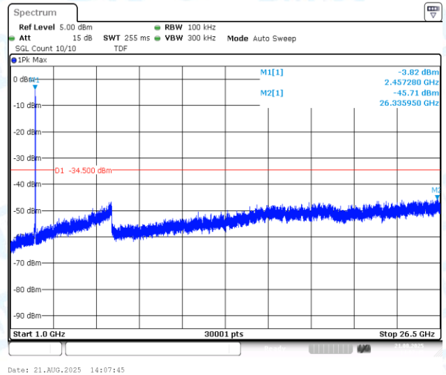
11AX20MIMO-Ant2-2462-1000~26500-PASS
