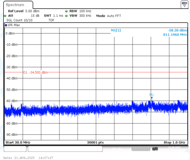
11AX20MIMO-Ant2-2462-30~1000-PASS
