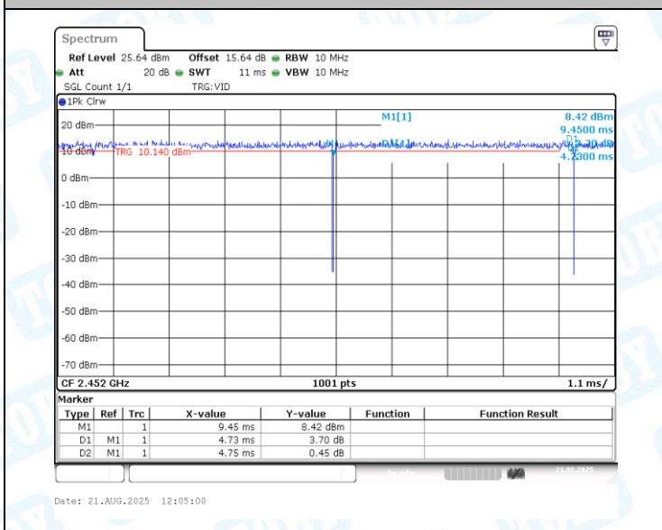
NTNV-11N40MIMO-Ant1-2452
