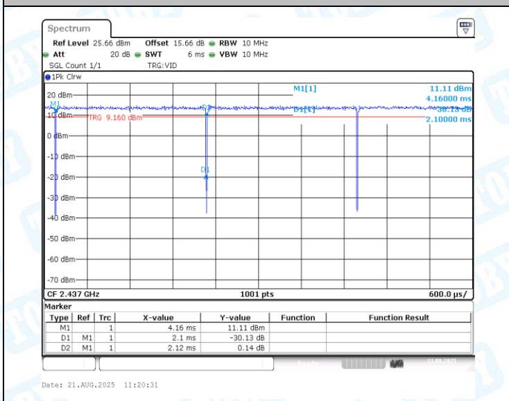
NTNV-11G-CDD-Ant1-2437
