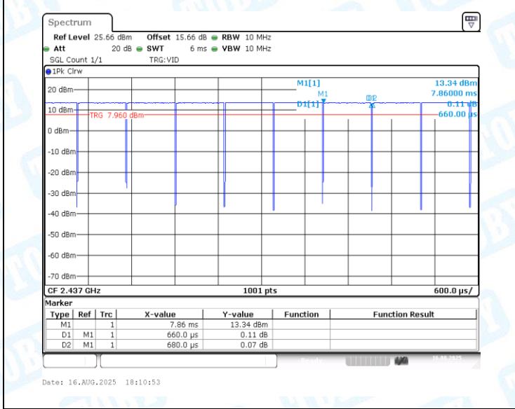
NTVN-11B-CDD-Ant1-2437
