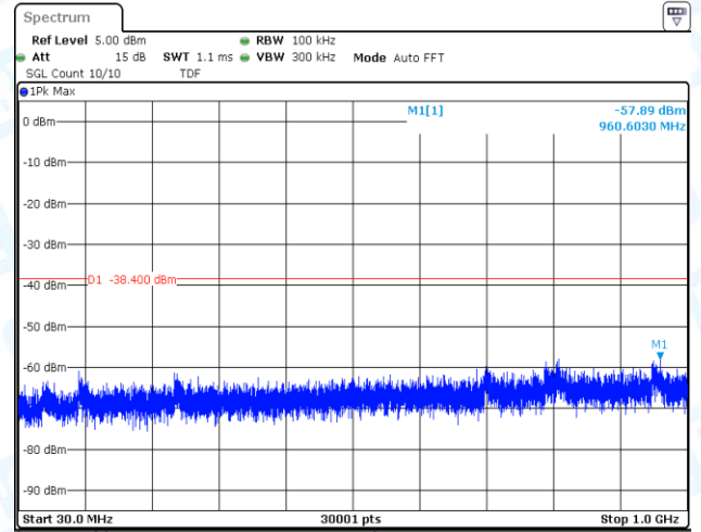
11AX40MIMO-Ant2-2452-0~Reference-PASS
