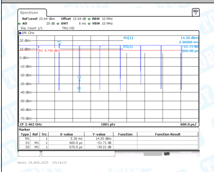
NTVN-11B-CDD-Ant1-2462
