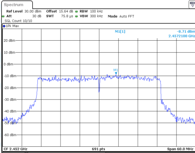
11AX40MIMO-Ant1-2452-0~Reference-PASS
