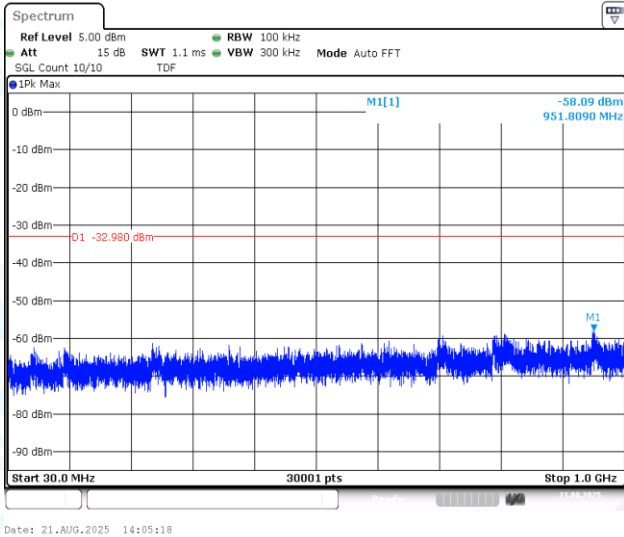
11AX20MIMO-Ant1-2462-30~1000-PASS
