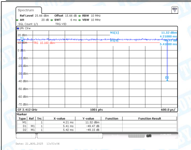
NTVN-11AX20MIMO-Ant1-2412
