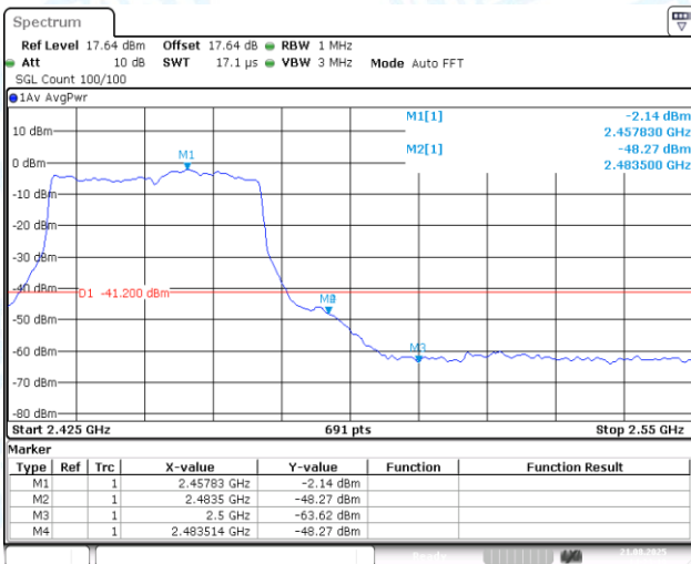
11AX40MIMO-Ant1-2452-PASS
