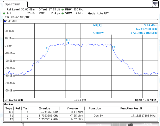
11A-CDD-Ant2-5745
