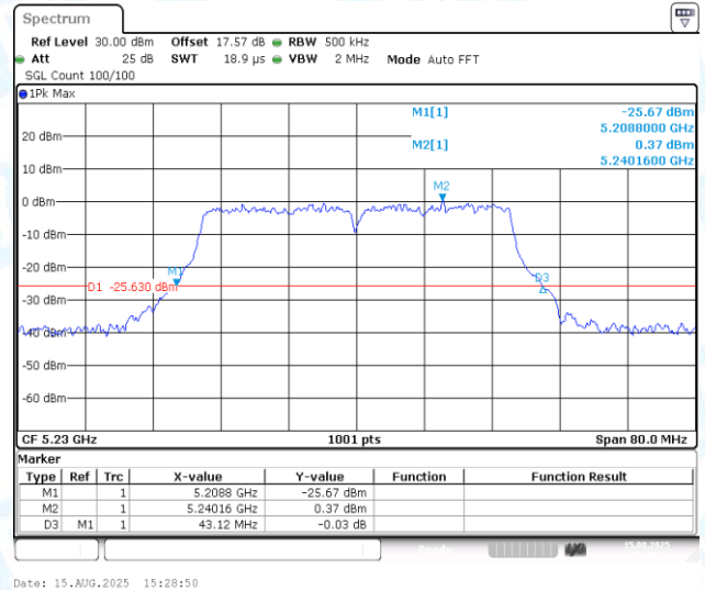
11AC40MIMO-Ant2-5230
