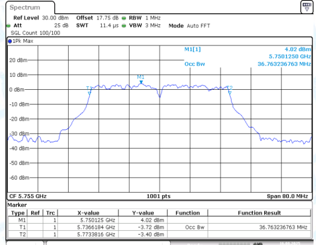
11AC40MIMO-Ant2-5755
