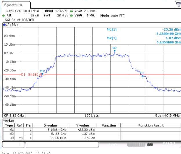
11A-CDD-Ant1-5180
