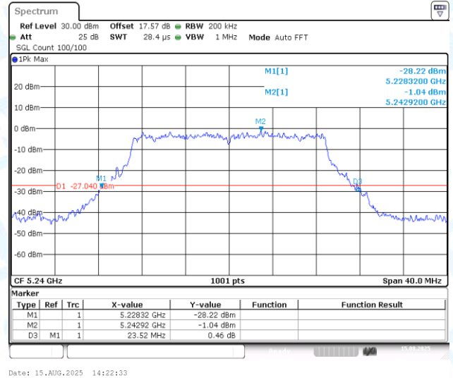
11N20MIMO-Ant2-5240
