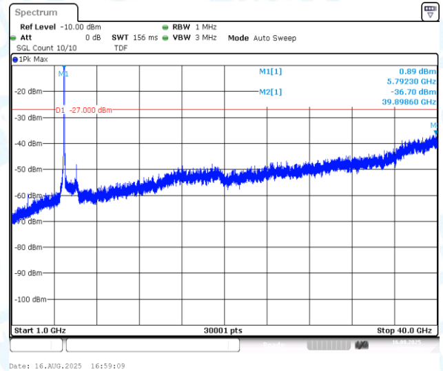
11AC80MIMO-Ant2-5775-1000~40000-PASS
