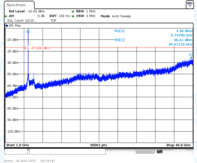
11AC40MIMO-Ant2-5755-1000~40000-PASS
