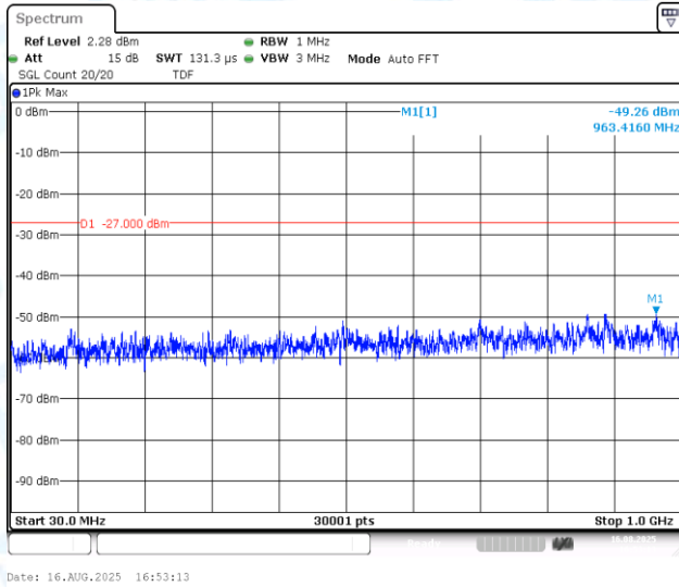
11AC80MIMO-Ant1-5775-30~1000-PASS
