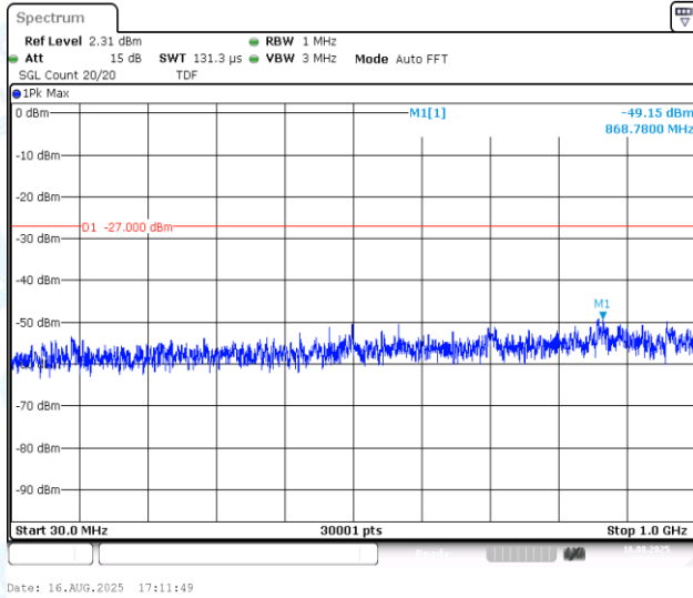
11AX20MIMO-Ant1-5785-30~1000-PASS
