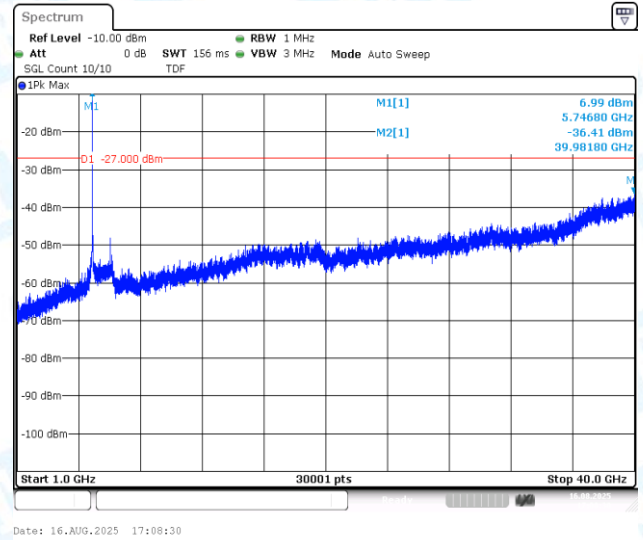
11AX20MIMO-Ant2-5745-1000~40000-PASS
