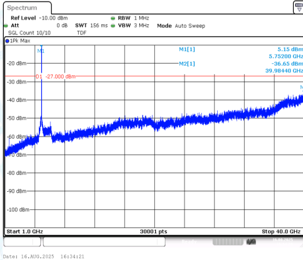
11AC40MIMO-Ant1-5755-1000~40000-PASS
