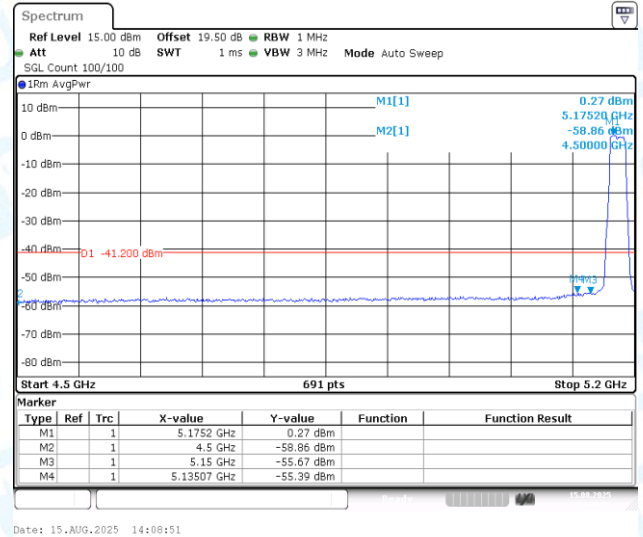
11N20MIMO-Ant2-5180-PASS
