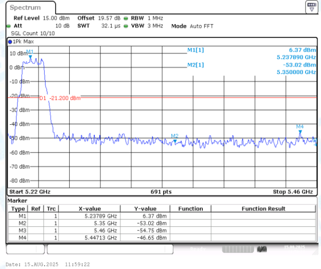
11A-CDD-Ant2-5240-PASS
