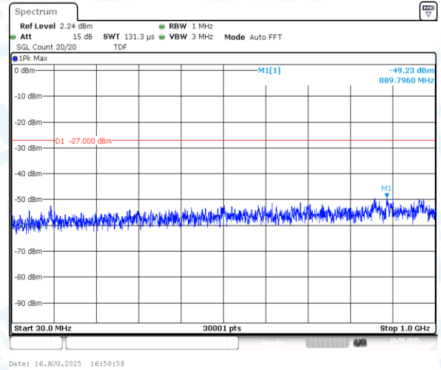
11AC80MIMO-Ant2-5775-30~1000-PASS
