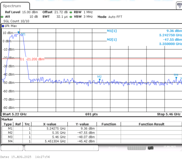
11N20MIMO-Ant1-5240-PASS
