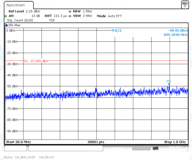
11AC40MIMO-Ant2-5755-30~1000-PASS
