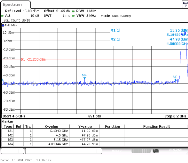
11N20MIMO-Ant1-5180-PASS
