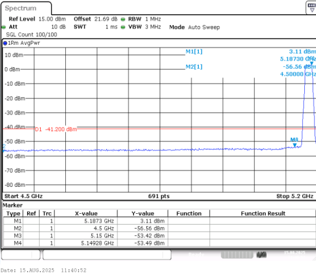
11A-CDD-Ant1-5180-PASS
