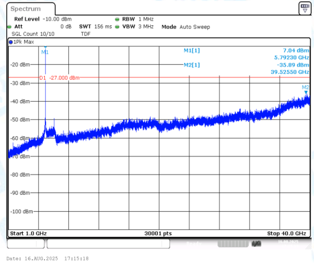
11AX20MIMO-Ant2-5785-1000~40000-PASS
