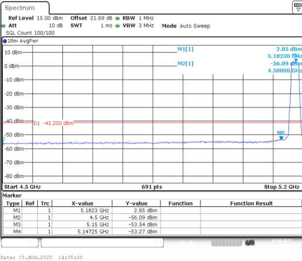
11N20MIMO-Ant1-5180-PASS
