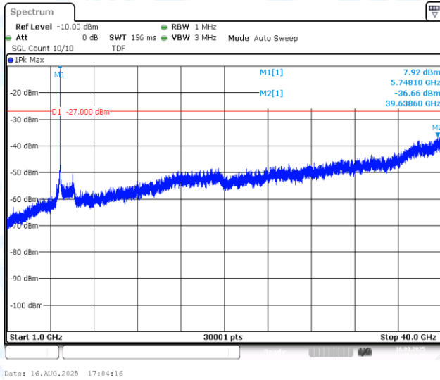
11AX20MIMO-Ant1-5745-1000~40000-PASS
