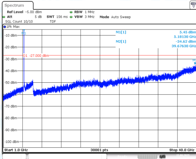
11AX40MIMO-Ant1-5190-1000~40000-PASS
