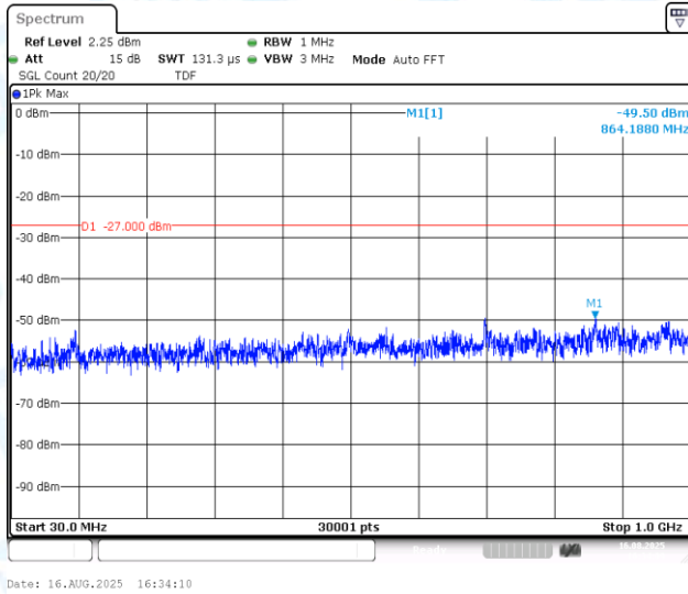
11AC40MIMO-Ant1-5755-30~1000-PASS
