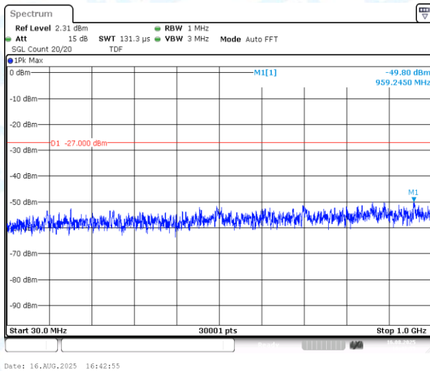
11AC40MIMO-Ant1-5795-30~1000-PASS
