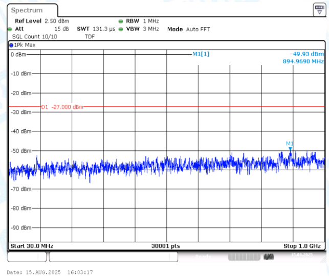
11AX20MIMO-Ant2-5180-30~1000-PASS
