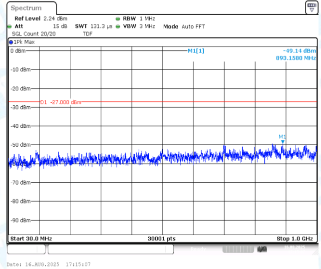
11AX20MIMO-Ant2-5785-30~1000-PASS
