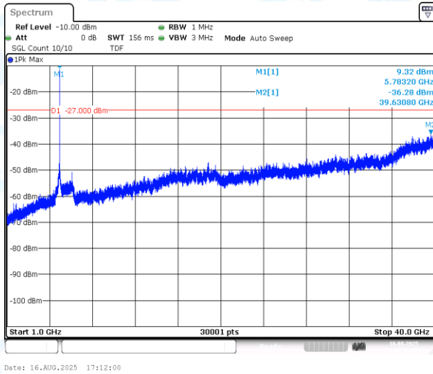
11AX20MIMO-Ant1-5785-1000~40000-PASS
