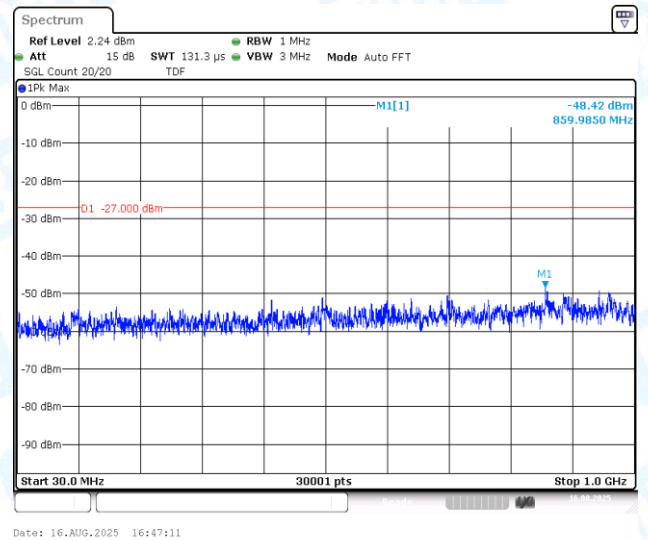
11AC40MIMO-Ant2-5795-30~1000-PASS
