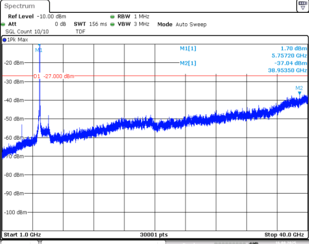
11AX80MIMO-Ant2-5775-1000~40000-PASS
