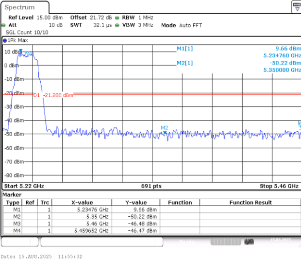
11A-CDD-Ant1-5240-PASS
