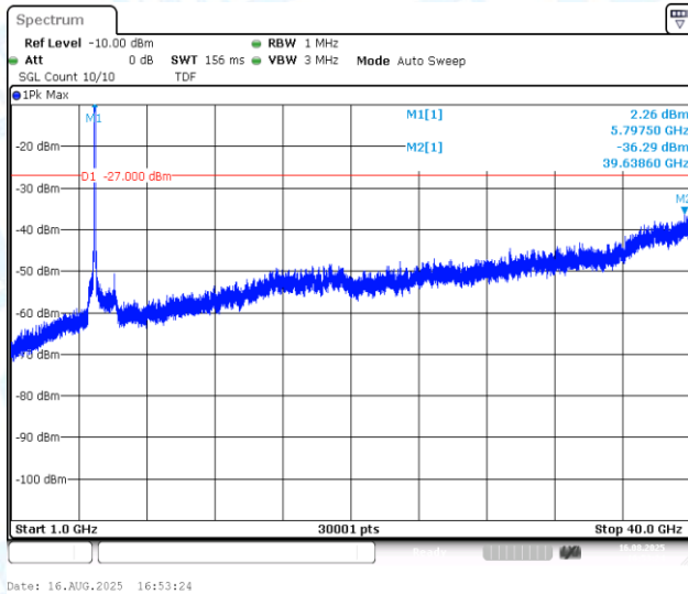
11AC80MIMO-Ant1-5775-1000~40000-PASS
