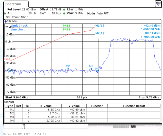
11N40MIMO-Ant2-5755-PASS
