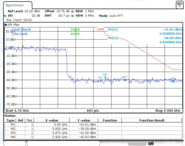
11AX80MIMO-Ant1-5775-PASS
