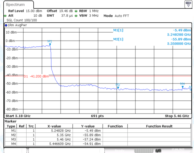
11AX80MIMO-Ant2-5210-PASS
