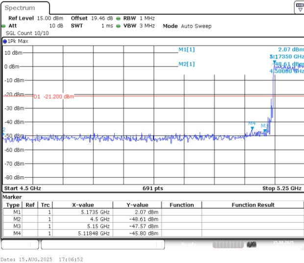
11AX80MIMO-Ant2-5210-PASS
