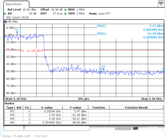
11AX80MIMO-Ant2-5210-PASS
