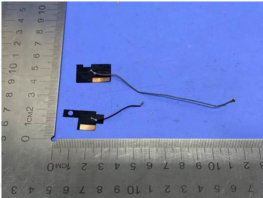
Photo 14 Internal of Antenna
