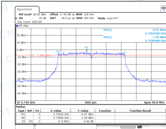
11N20MIMO-Ant1-5745-PASS
