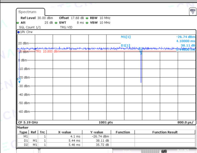
NTNV-11AC40MIMO-Ant2-5190
