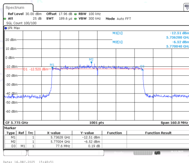
11AX80MIMO-Ant2-5775-PASS
