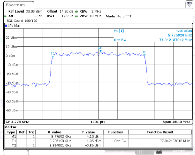
11AX80MIMO-Ant2-5775
