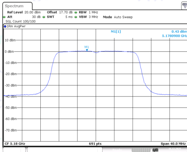
11N20MIMO-Ant2-5180-PASS
