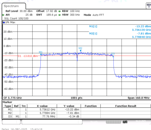
11AX80MIMO-Ant1-5775-PASS
