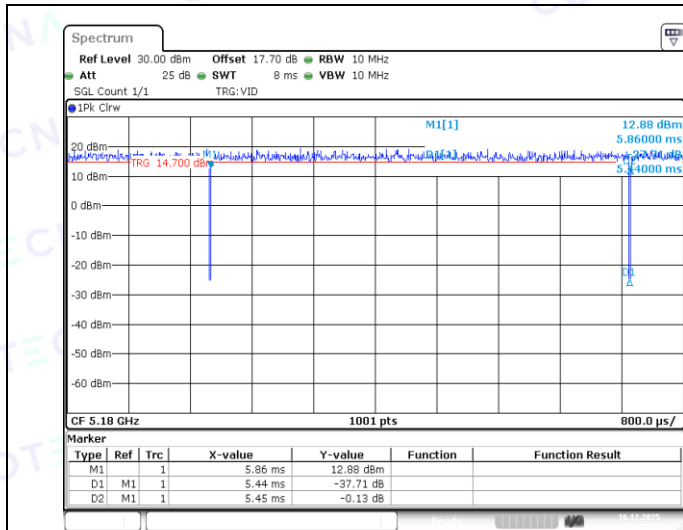
NTNV-11AC20MIMO-Ant2-5180
