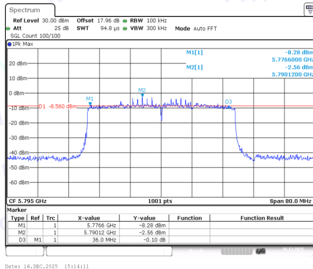
11AX40MIMO-Ant2-5795-PASS
