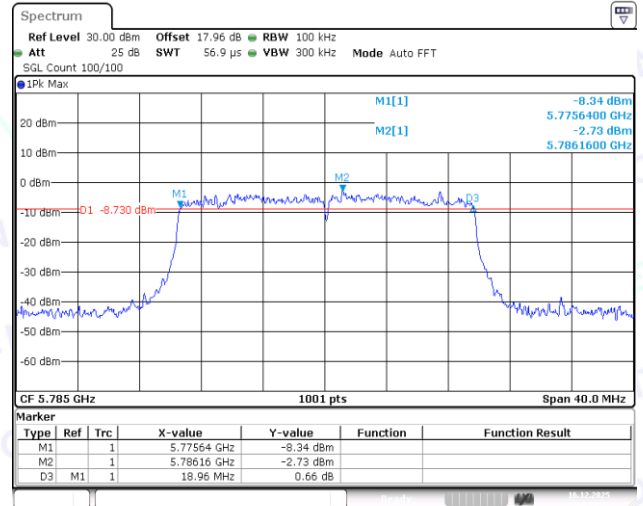
11AX20MIMO-Ant2-5785-PASS
