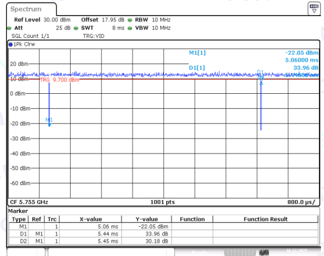
NTNV-11AC40MIMO-Ant2-5755
