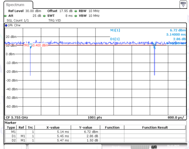
NTNV-11AX40MIMO-Ant2-5755
