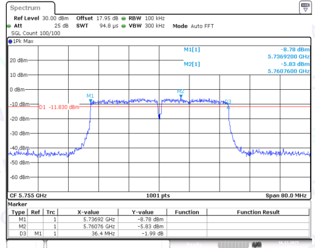
11N40MIMO-Ant2-5755-PASS
