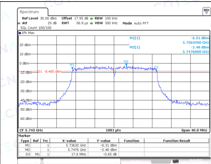
11N20MIMO-Ant2-5745-PASS
