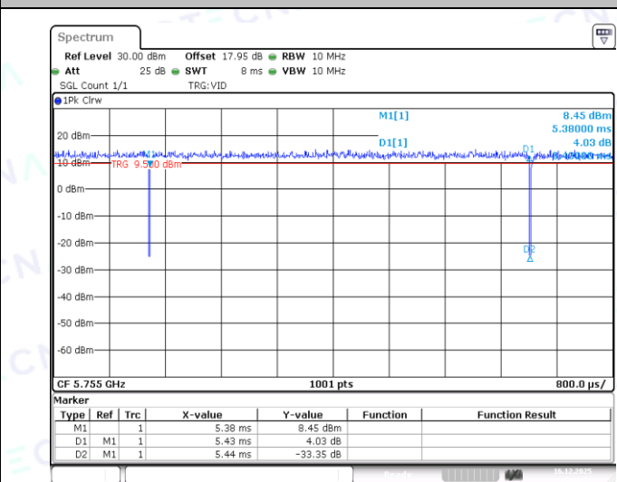
NTNV-11N40MIMO-Ant2-5755
