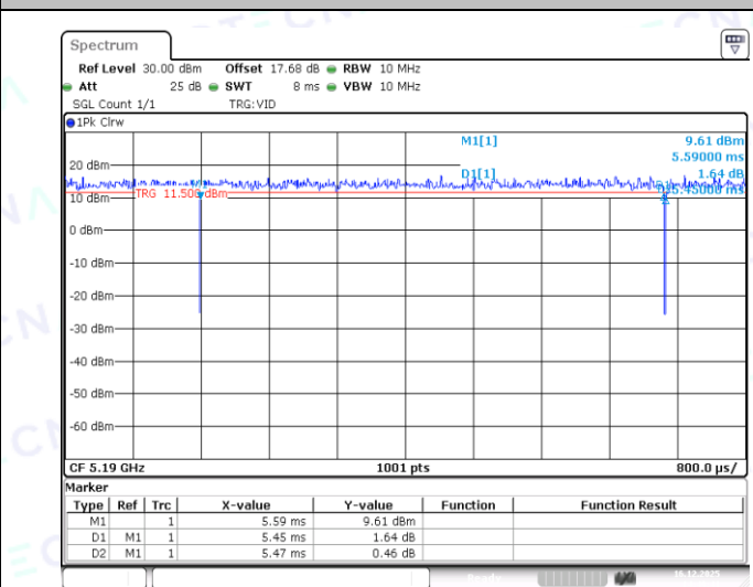
NTNV-11AX40MIMO-Ant2-5190
