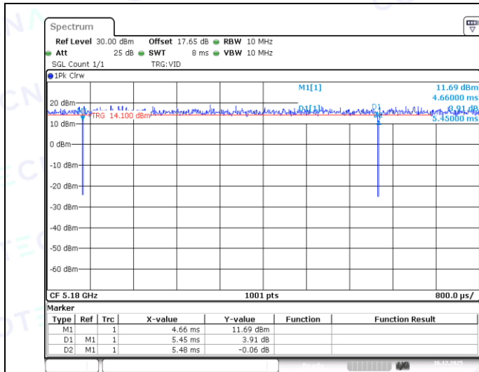
NTNV-11AX20MIMO-Ant1-5180
