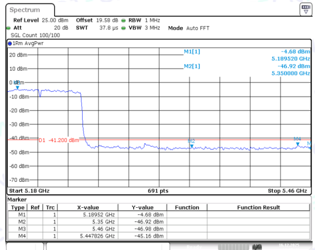
11AC80MIMO-Ant2-5210-PASS
