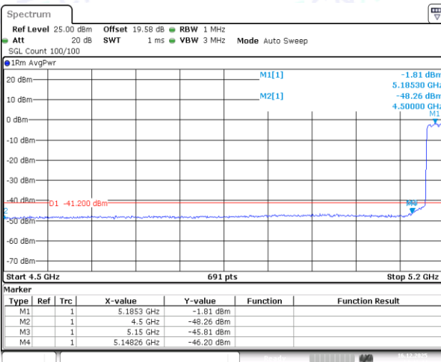
11AX40MIMO-Ant1-5190-PASS
