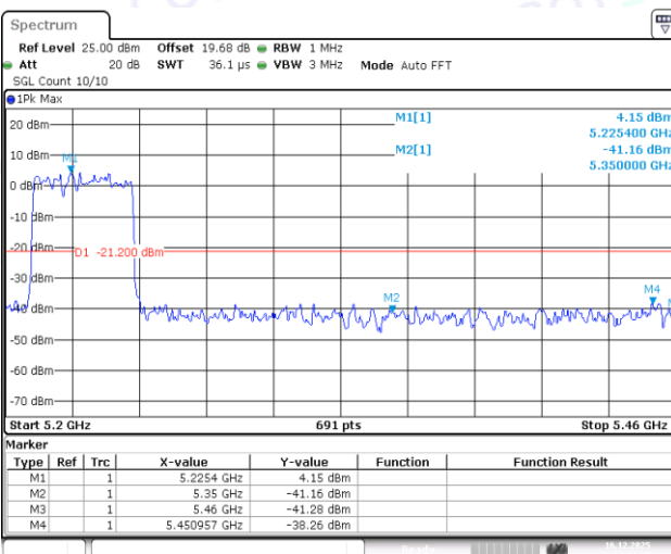
11AX40MIMO-Ant1-5190-PASS
