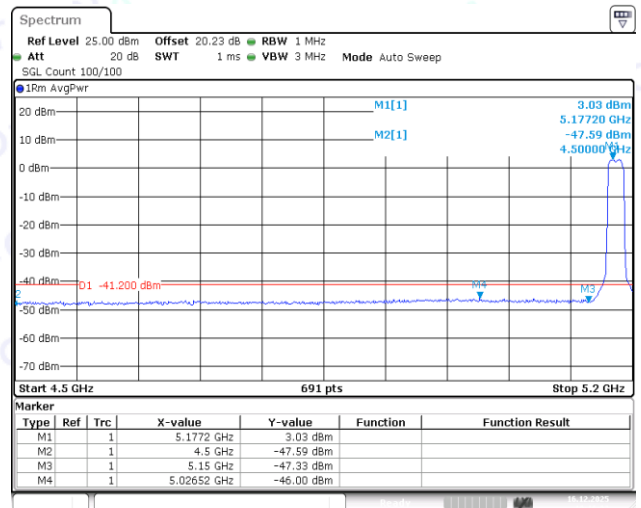
11AC20MIMO-Ant2-5180-PASS
