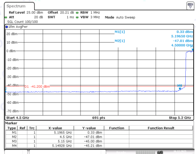
11AX40MIMO-Ant2-5190-PASS
