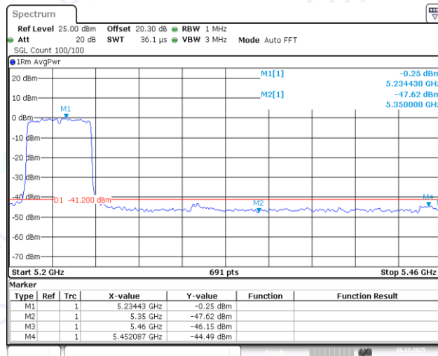
11AX40MIMO-Ant2-5230-PASS
