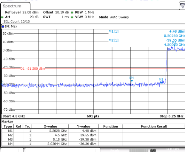
11AC80MIMO-Ant1-5210-PASS
