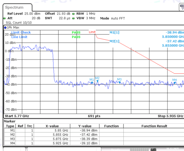
11AX40MIMO-Ant2-5755-PASS
