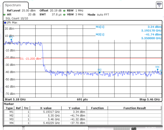
11AC80MIMO-Ant1-5210-PASS
