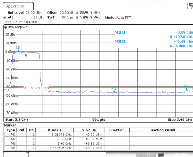
11AC40MIMO-Ant2-5230-PASS
