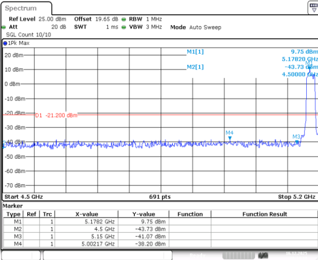
11AC20MIMO-Ant1-5180-PASS
