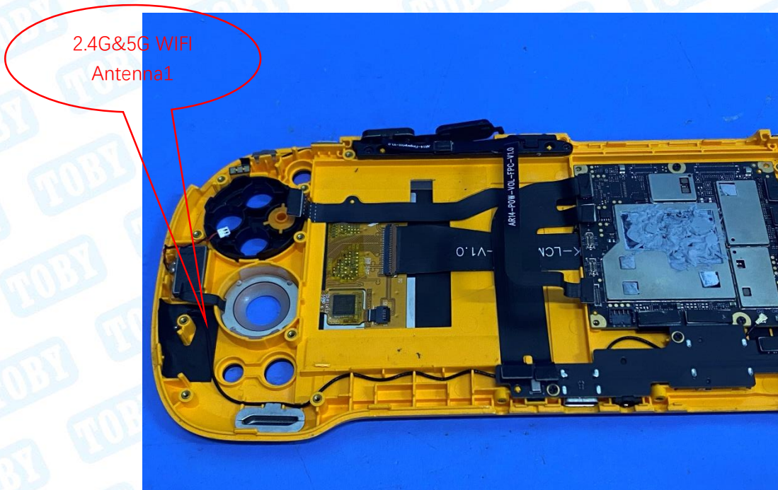
Photo 16 Internal of EUT
