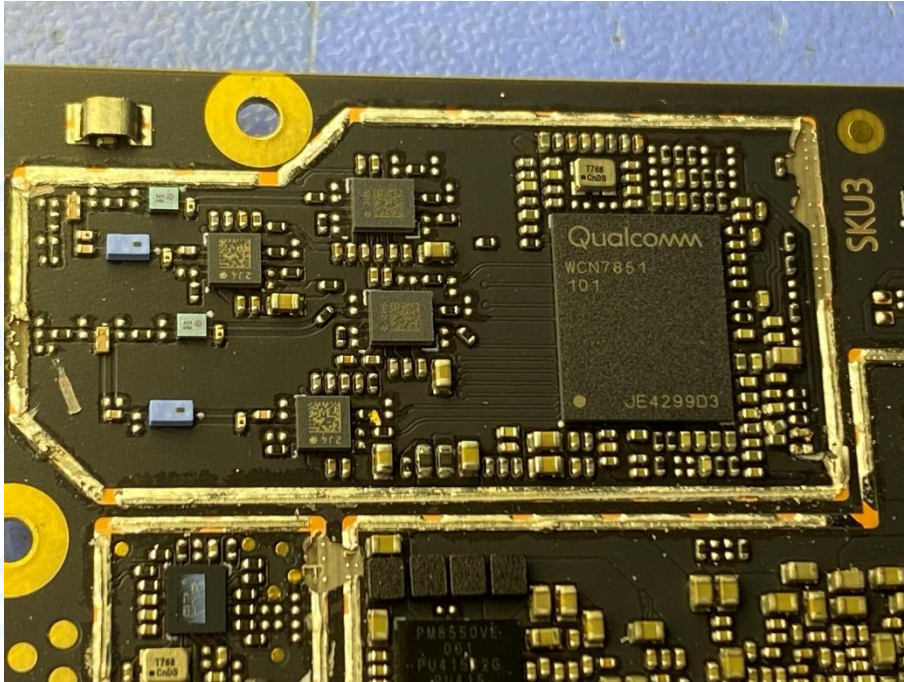
Photo 31 Appearance of PCB
