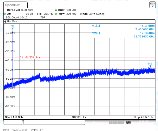
11AX40MIMO-Ant2-2452-1000~26500-PASS
