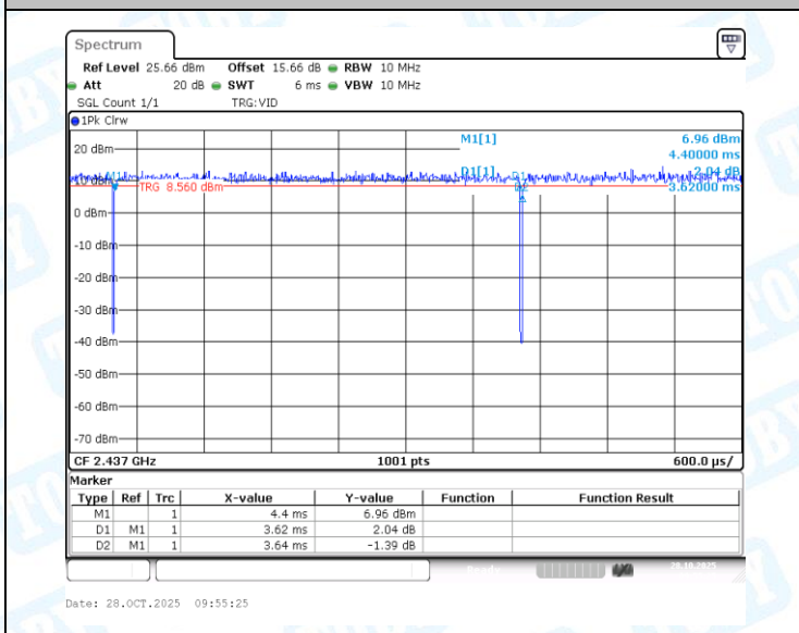
NTVN-11AX40MIMO-Ant1-2437
