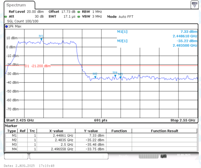
11AX40MIMO-Ant2-2452-PASS
