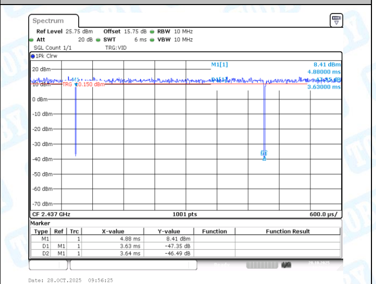
NTVN-11AX40MIMO-Ant2-2437
