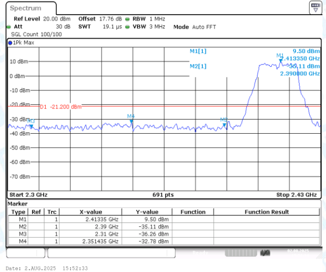
11G-CDD-Ant2-2412-PASS
