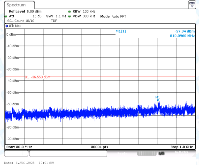
11AX40MIMO-Ant2-2452-30~1000-PASS
