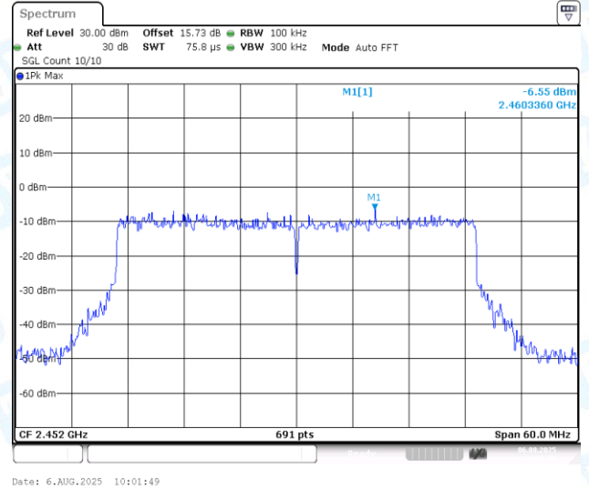
11AX40MIMO-Ant2-2452-0~Reference-PASS
