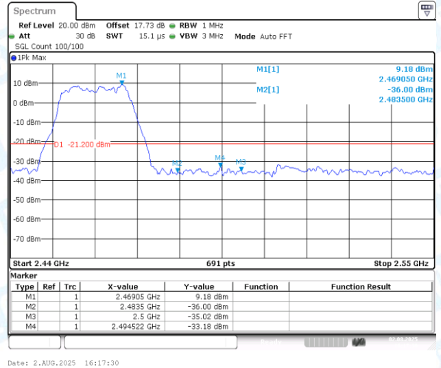
11N20MIMO-Ant2-2462-PASS
