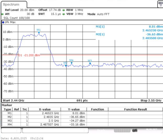
11G-CDD-Ant1-2462-PASS
