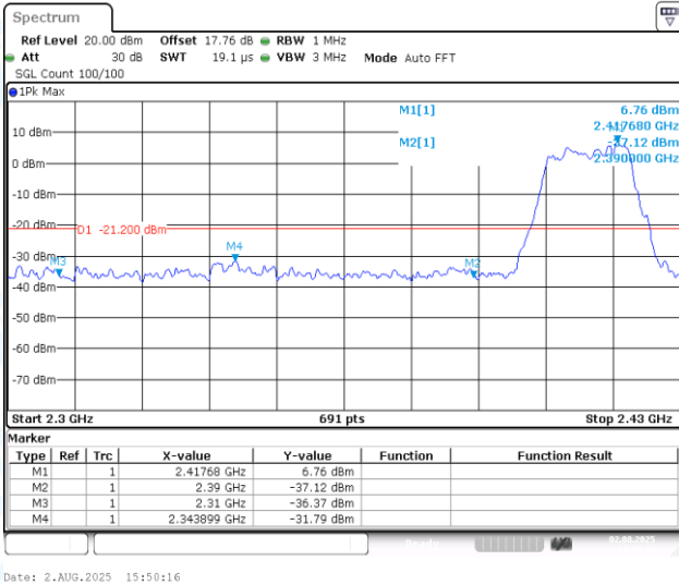
11G-CDD-Ant1-2412-PASS
