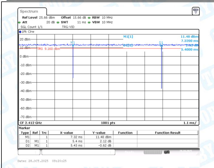
NTNV-11N20MIMO-Ant1-2412
