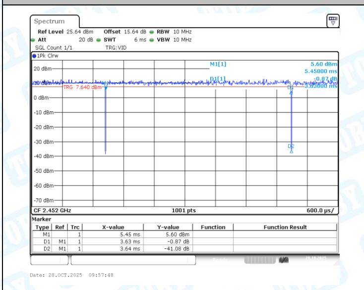
NTVN-11AX40MIMO-Ant1-2452
