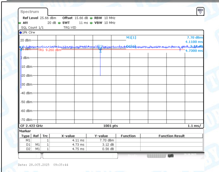
NTNV-11N40MIMO-Ant1-2422
