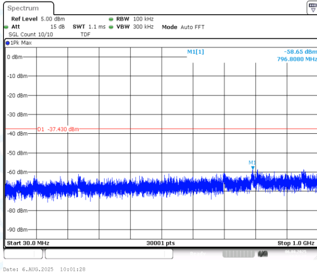
11AX40MIMO-Ant1-2452-30~1000-PASS
