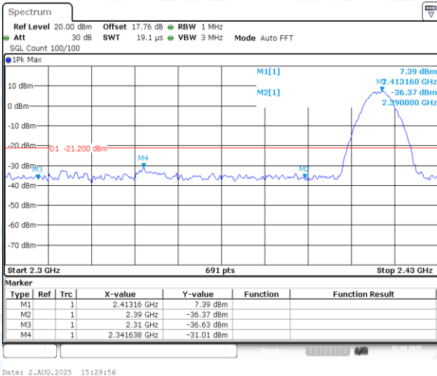
11B-CDD-Ant1-2412-PASS
