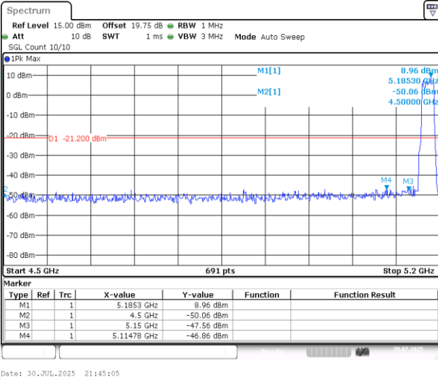
11AX20MIMO-Ant1-5180-PASS
