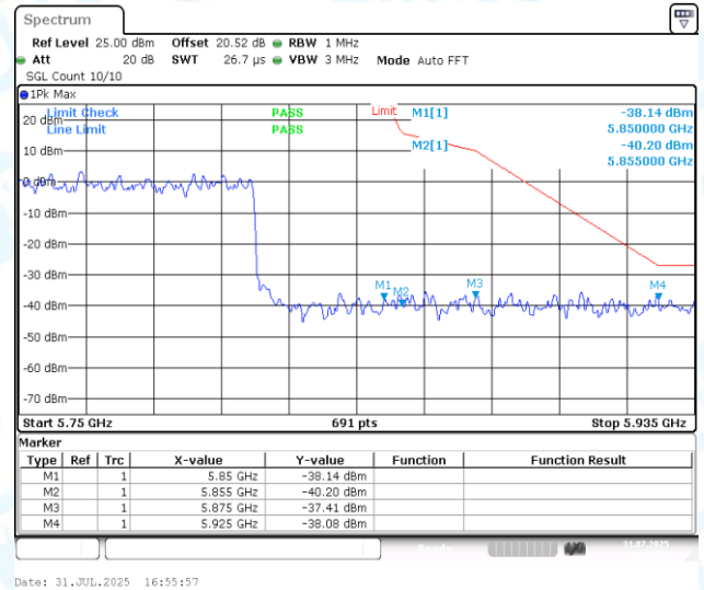
11AX80MIMO-Ant1-5775-PASS
