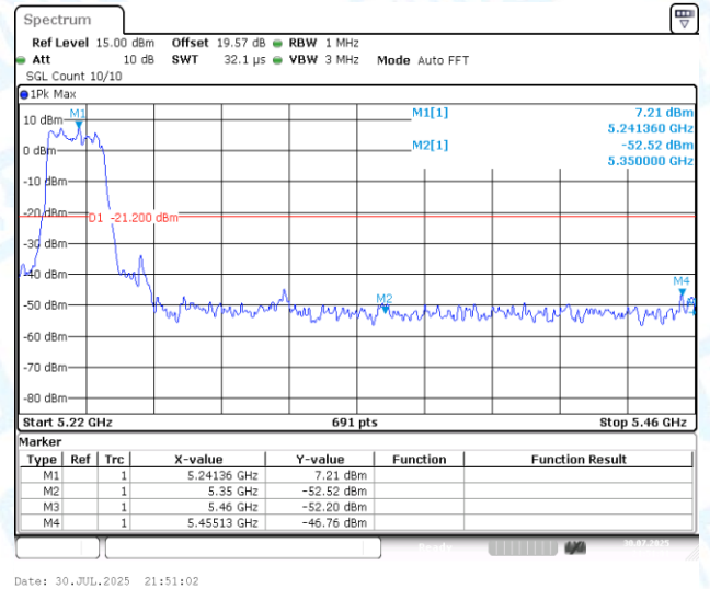
11AX20MIMO-Ant2-5240-PASS
