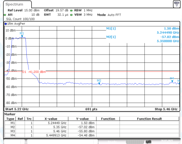
11AX20MIMO-Ant2-5240-PASS
