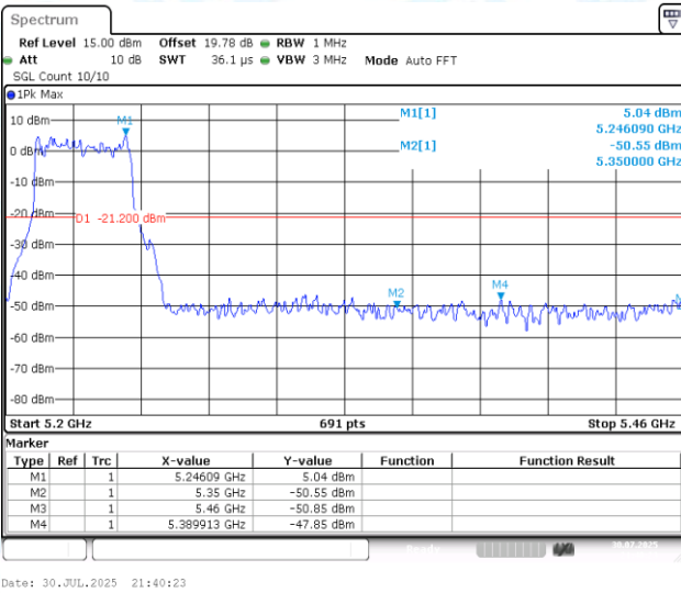
11AC40MIMO-Ant1-5230-PASS
