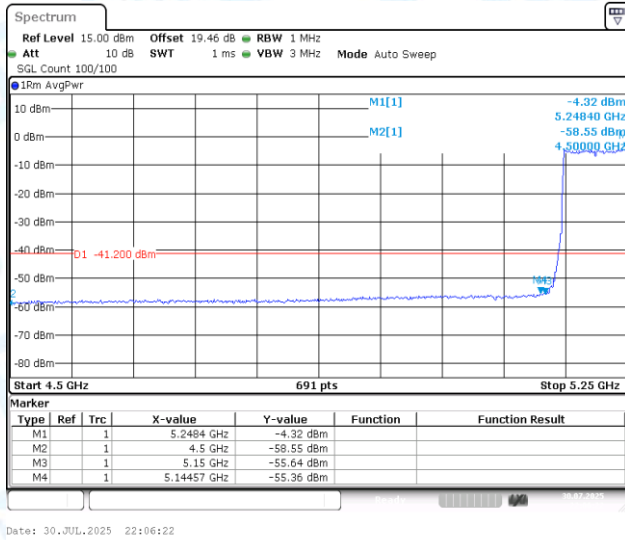
11AX80MIMO-Ant2-5210-PASS
