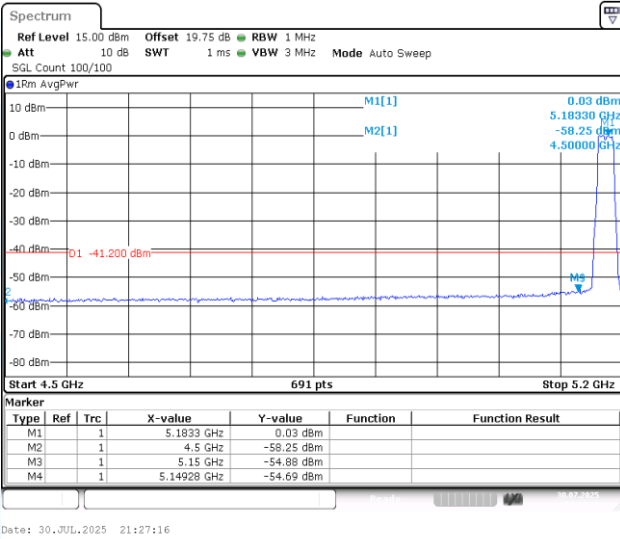
11AC20MIMO-Ant1-5180-PASS
