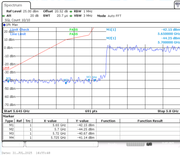
11AX80MIMO-Ant1-5775-PASS
