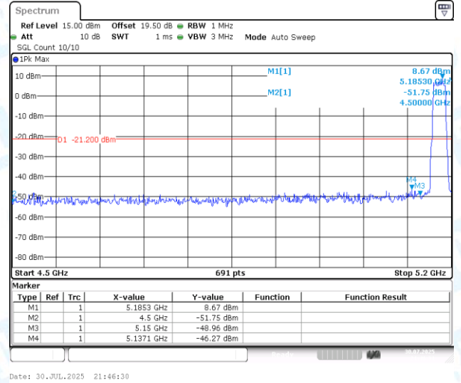
11AX20MIMO-Ant2-5180-PASS
