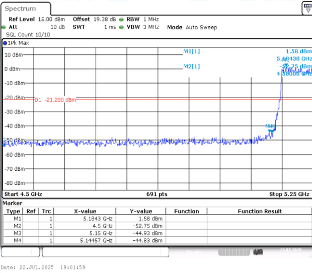
11AC80MIMO-Ant1-5210-PASS
