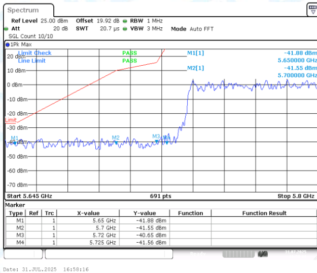
11AX80MIMO-Ant2-5775-PASS
