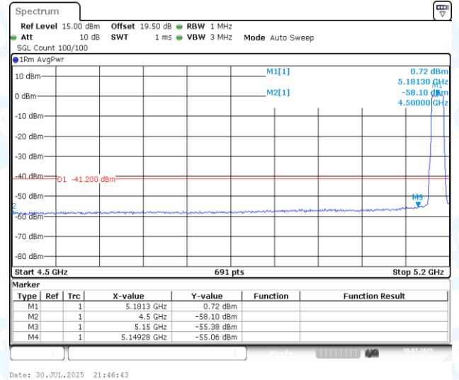
11AX20MIMO-Ant2-5180-PASS
