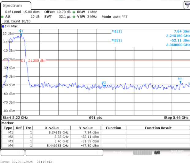
11AX20MIMO-Ant1-5240-PASS
