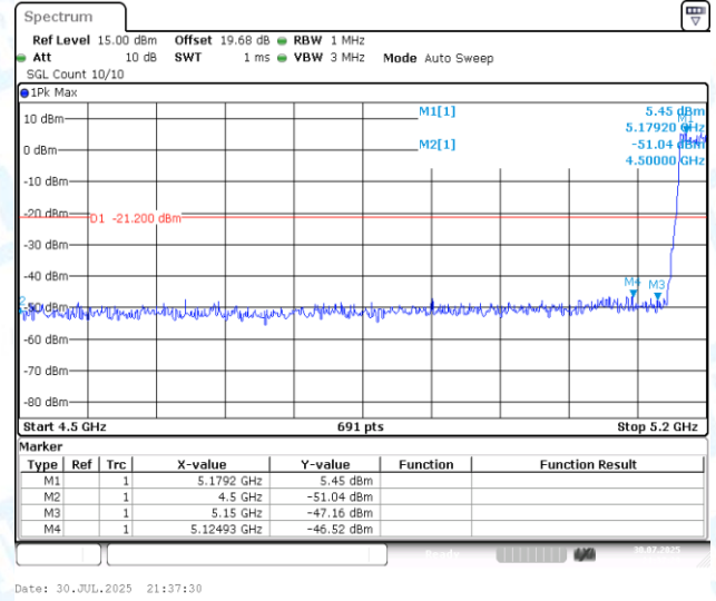
11AC40MIMO-Ant1-5190-PASS
