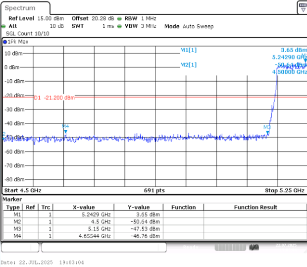
11AC80MIMO-Ant2-5210-PASS
