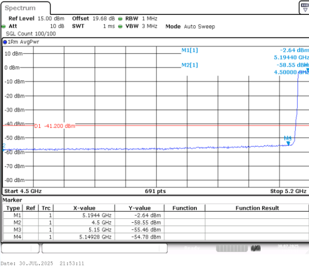
11AX40MIMO-Ant1-5190-PASS
