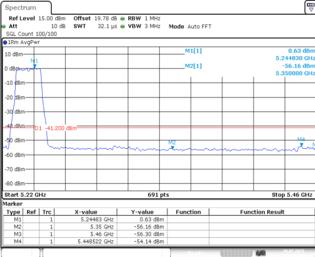
11AX20MIMO-Ant1-5240-PASS
