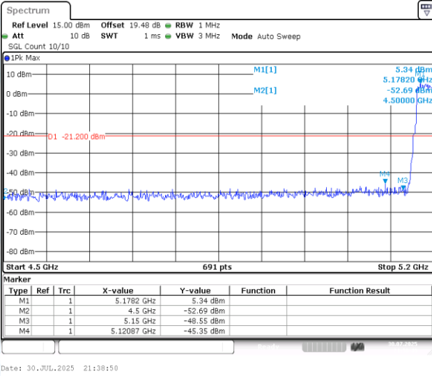
11AC40MIMO-Ant2-5190-PASS
