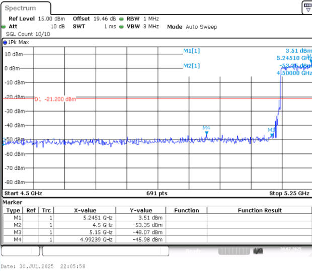
11AX80MIMO-Ant2-5210-PASS
