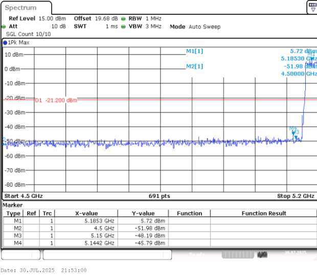
11AX40MIMO-Ant1-5190-PASS
