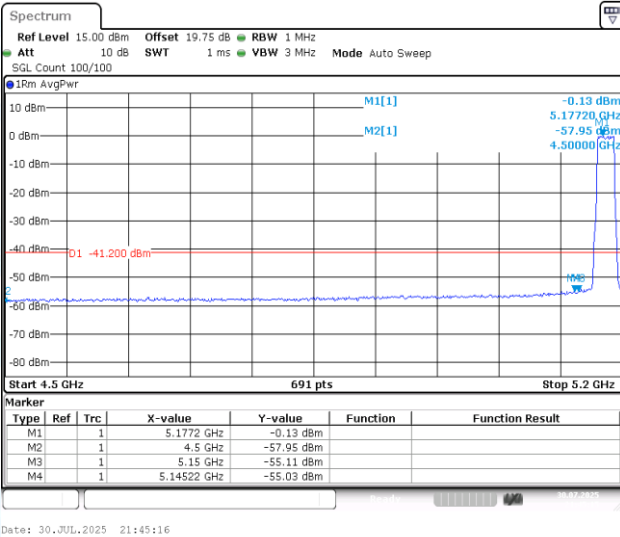
11AX20MIMO-Ant1-5180-PASS
