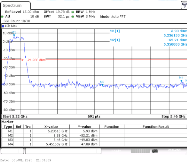
11AC20MIMO-Ant1-5240-PASS
