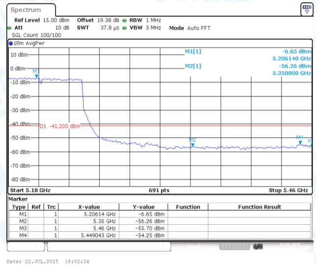
11AC80MIMO-Ant1-5210-PASS
