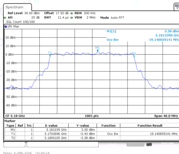
11AX20MIMO-Ant2-5180
