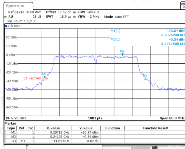
11AC40MIMO-Ant2-5230
