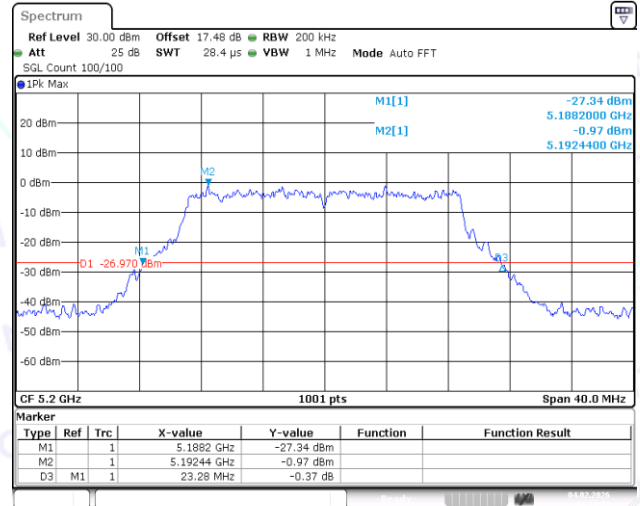
11AC20MIMO-Ant2-5200
