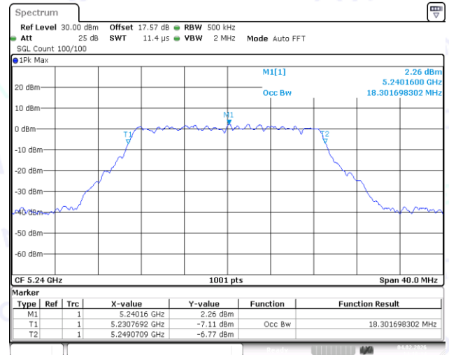
11AC20MIMO-Ant2-5240
