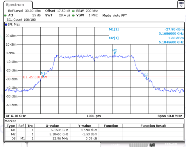
11N20MIMO-Ant2-5180
