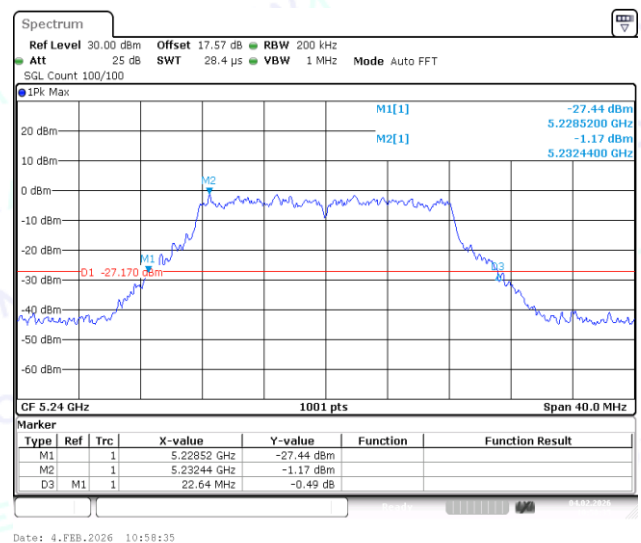
11A-CDD-Ant2-5240
