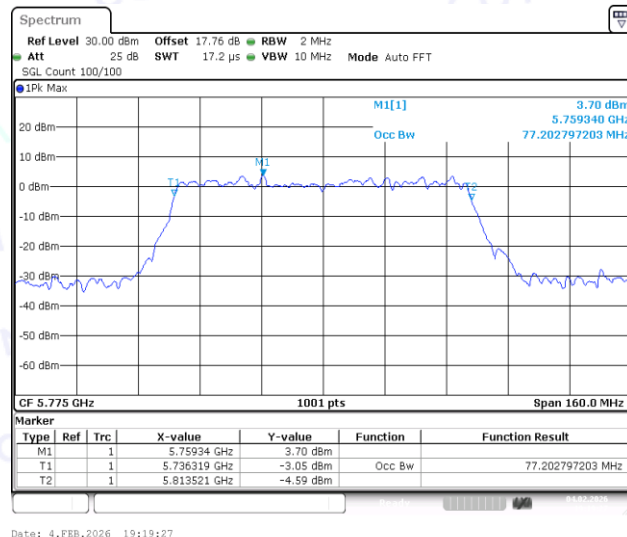
11AC80MIMO-Ant2-5775
