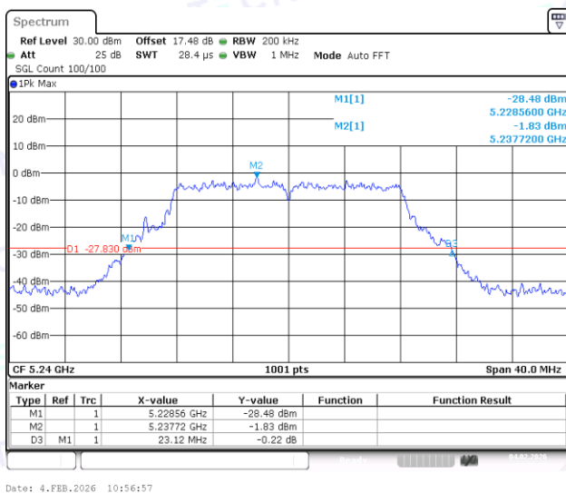
11A-CDD-Ant1-5240
