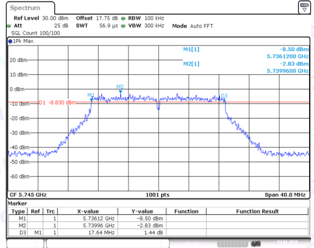
11N20MIMO-Ant2-5745-PASS
