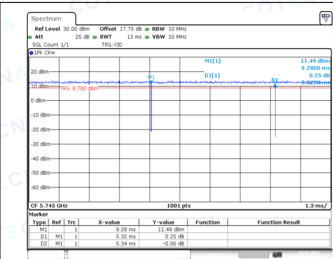
NTNV-11N20MIMO-Ant2-5745
