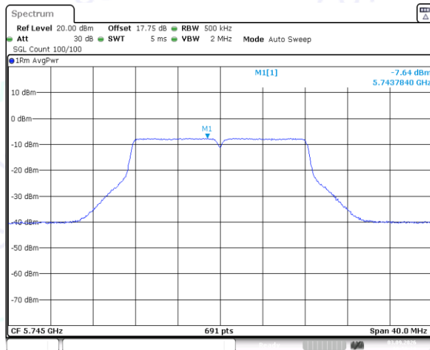
11A-CDD-Ant2-5745-PASS
