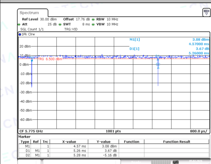
NTNV-11AX80MIMO-Ant2-5775
