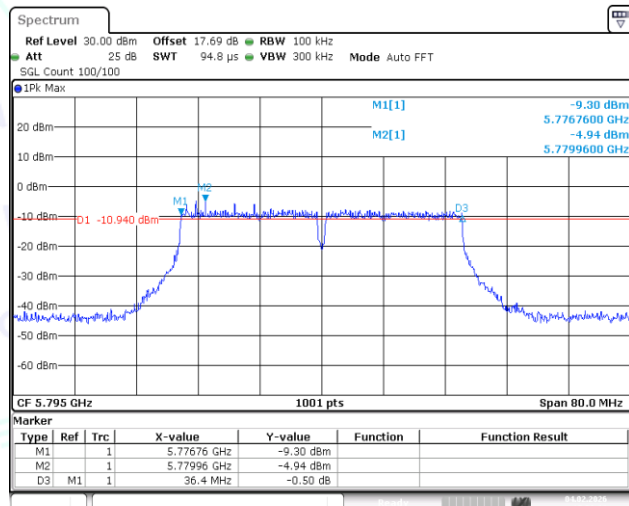
11AC40MIMO-Ant1-5795-PASS
