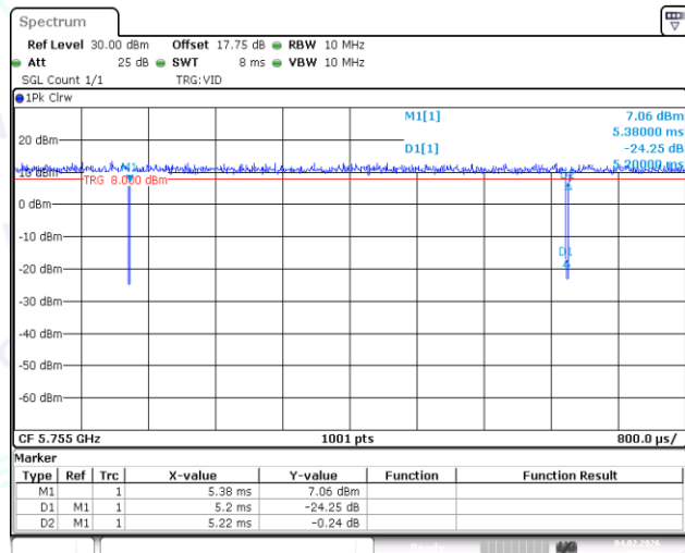
NTNV-11AC40MIMO-Ant1-5755
