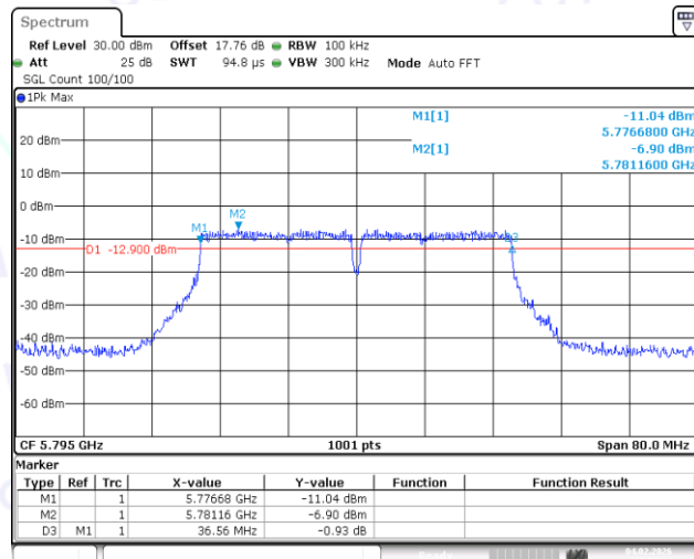
11AC40MIMO-Ant2-5795-PASS
