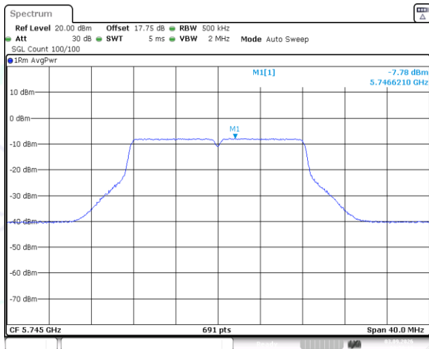
11A-CDD-Ant1-5745-PASS
