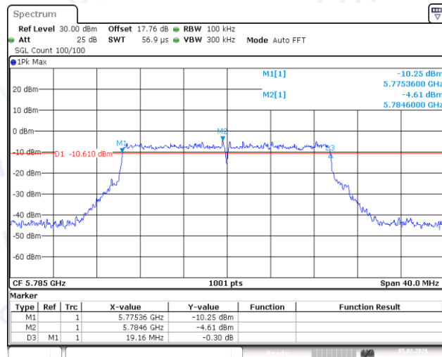
11AX20MIMO-Ant2-5785-PASS
