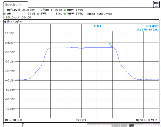
11N20MIMO-Ant2-5180-PASS
