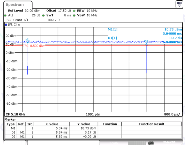
NTNV-11AX20MIMO-Ant2-5180
