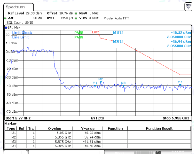
11AC40MIMO-Ant2-5755-PASS
