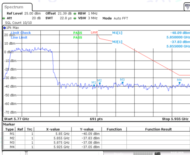
11AC40MIMO-Ant1-5755-PASS
