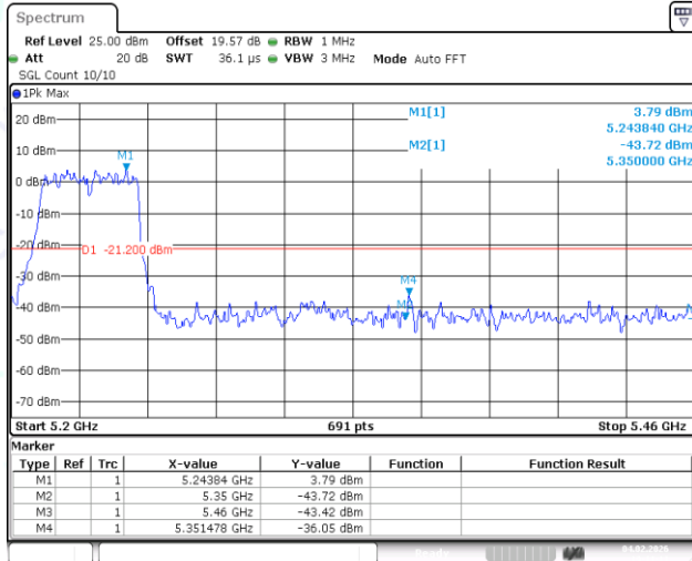
11AC40MIMO-Ant2-5230-PASS
