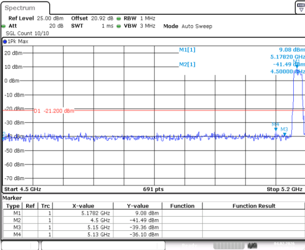
11AX20MIMO-Ant1-5180-PASS
