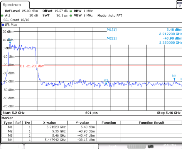
11AX40MIMO-Ant2-5230-PASS
