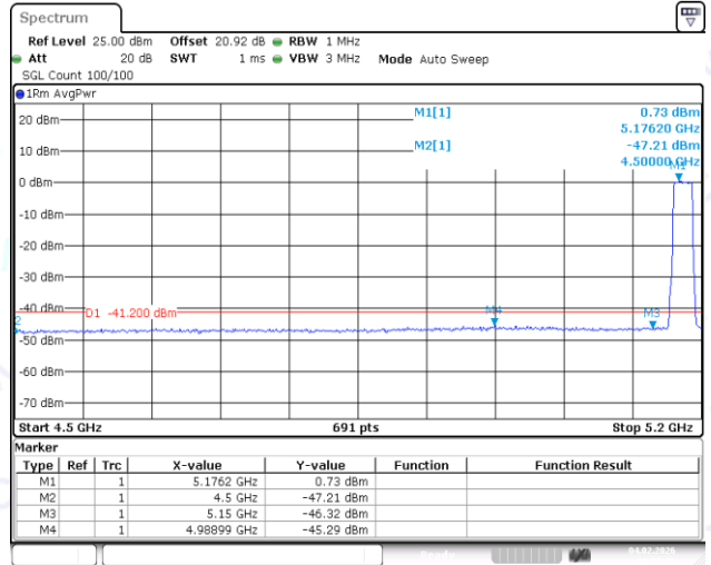
11AX20MIMO-Ant1-5180-PASS
