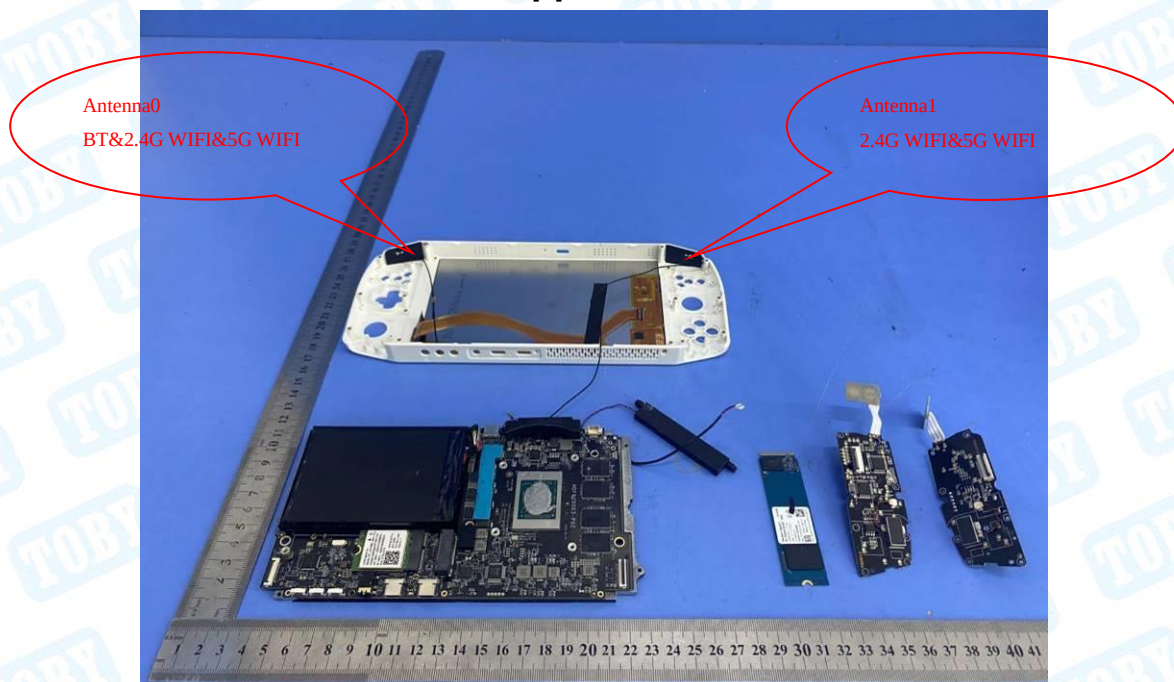
Photo 17 Appearance of PCB
