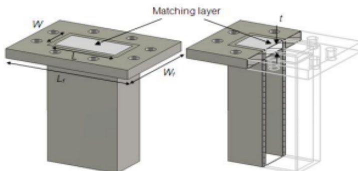
Figure 1: Validation Waveguide Dimensions
