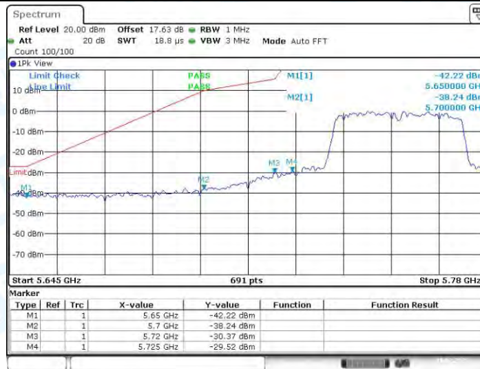
11AC40MIMO_Ant2_Low_5755_Peak
