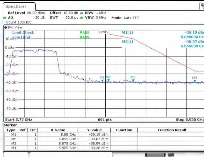
11AC40MIMO_Ant1_High_5795_Peak
