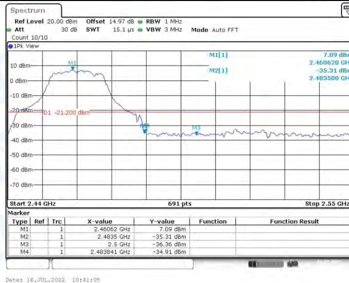
11N20MIMO_Ant0_High_2462_Peak
