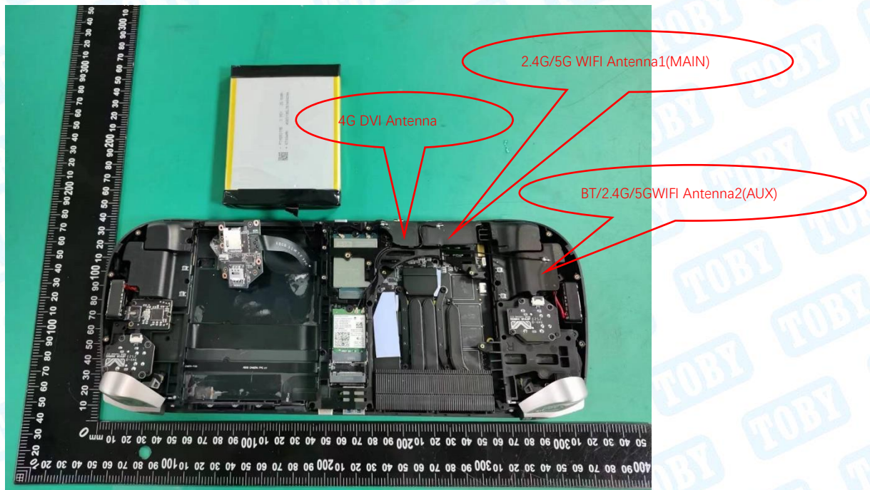
Photo 12 Internal of EUT
