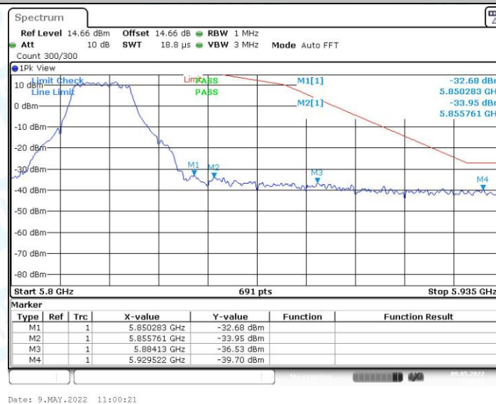
11AMIMO_Ant0_High_5825
