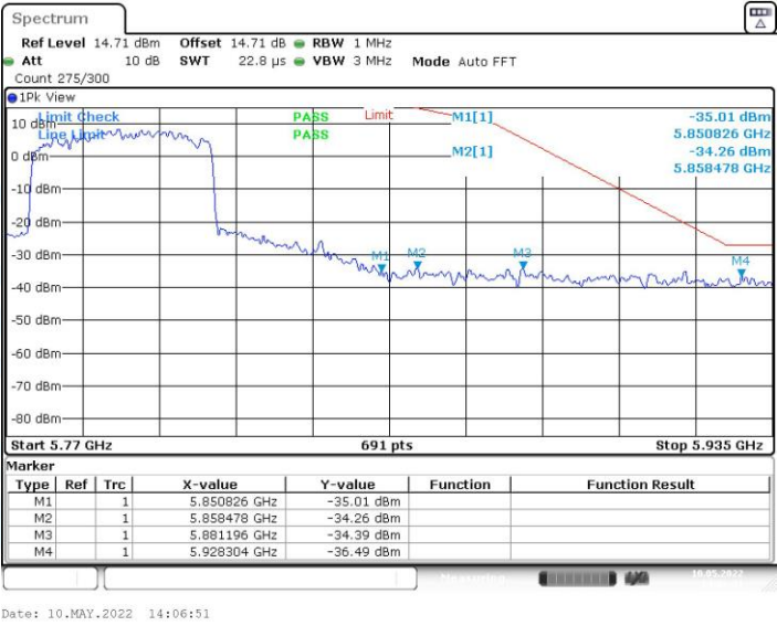
11AX40MIMO_Ant1_High_5795
