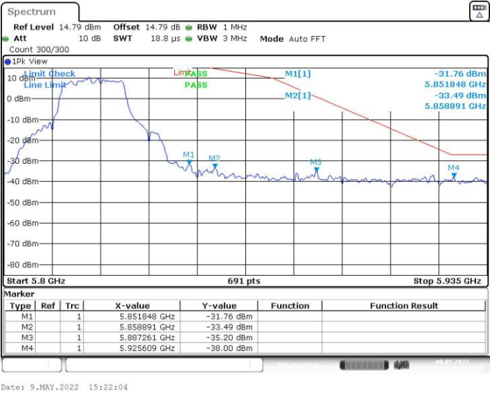
11N20MIMO_Ant1_High_5825
