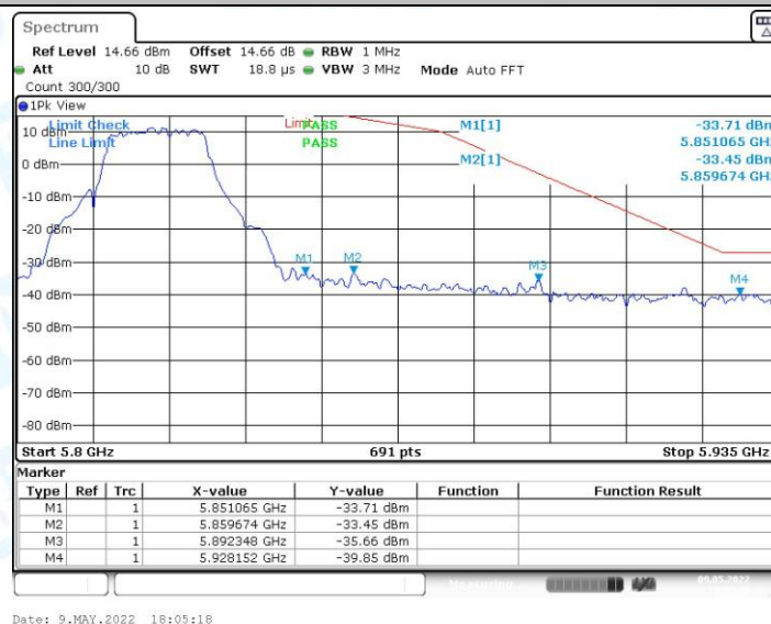
11AC20MIMO_Ant0_High_5825
