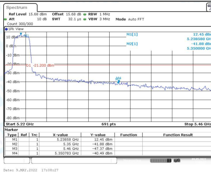
11AC20MIMO_Ant0_High_5240_Peak
