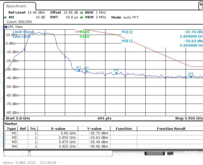
11N20MIMO_Ant0_High_5825_Peak
