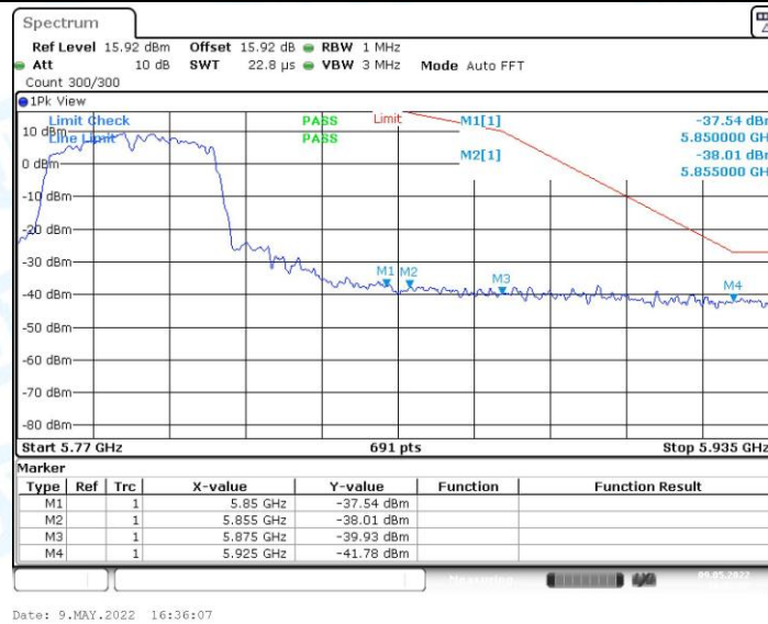
11N40MIMO_Ant0_High_5795_Peak
