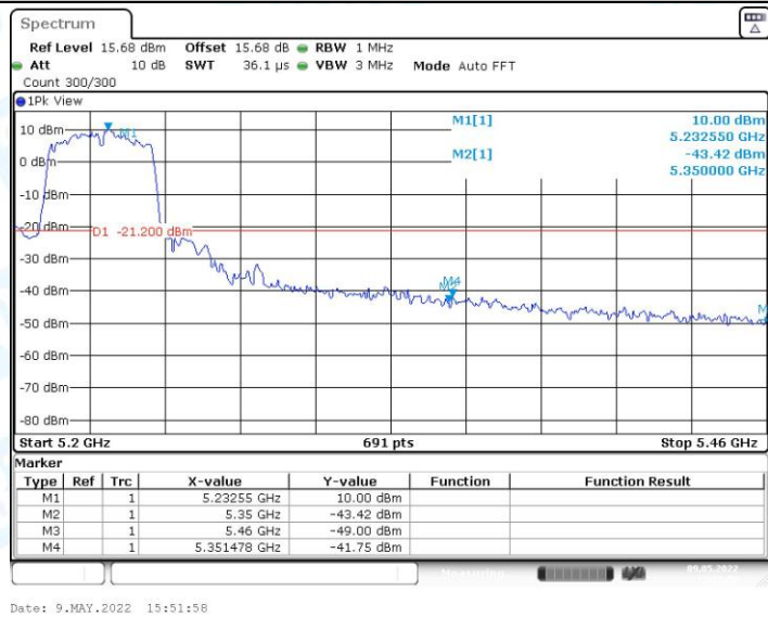
11N40MIMO_Ant0_High_5230_Peak
