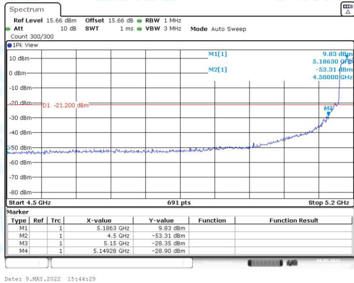
11N40MIMO_Ant1_Low_5190_Peak
