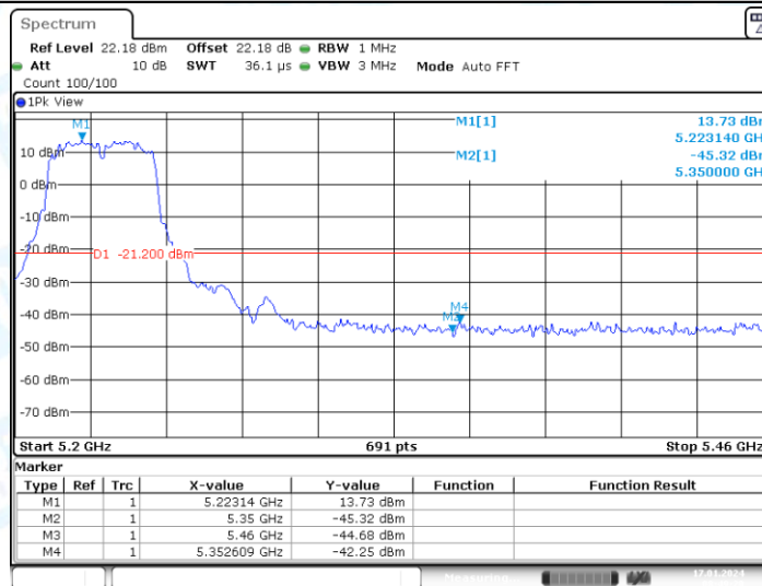
11N40MIMO_Ant2_High_5230_Peak
