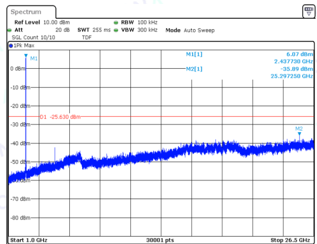
11B-Ant1-2437-0~Reference-PASS
