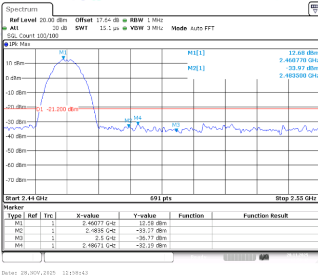
11B-Ant1-2462-PASS
