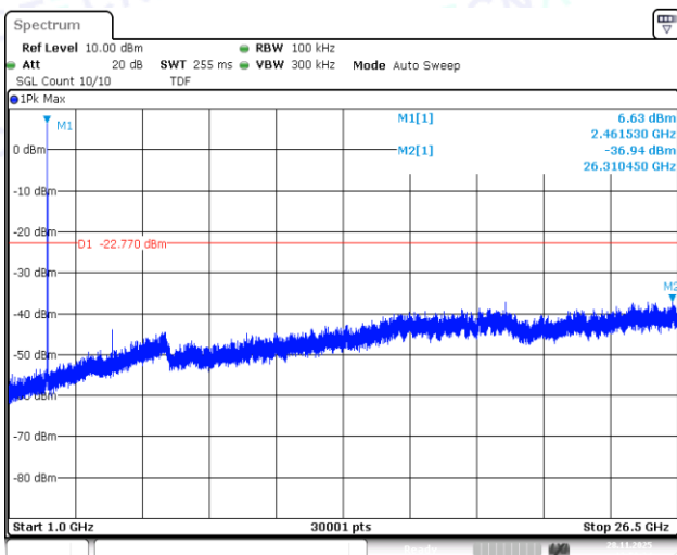
11B-Ant1-2462-0~Reference-PASS
