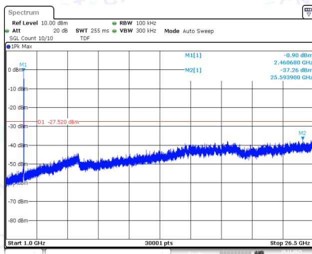
11G-Ant1-2462-0~Reference-PASS
