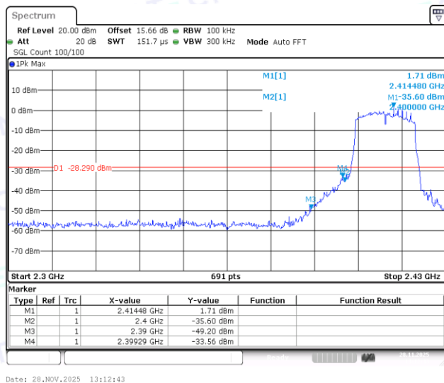
11N20SISO-Ant1-2412-PASS
