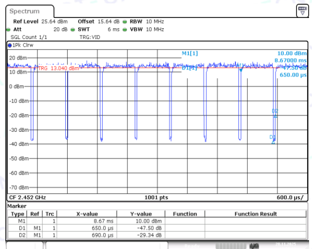
NTNV-11N40SISO-Ant1-2452
