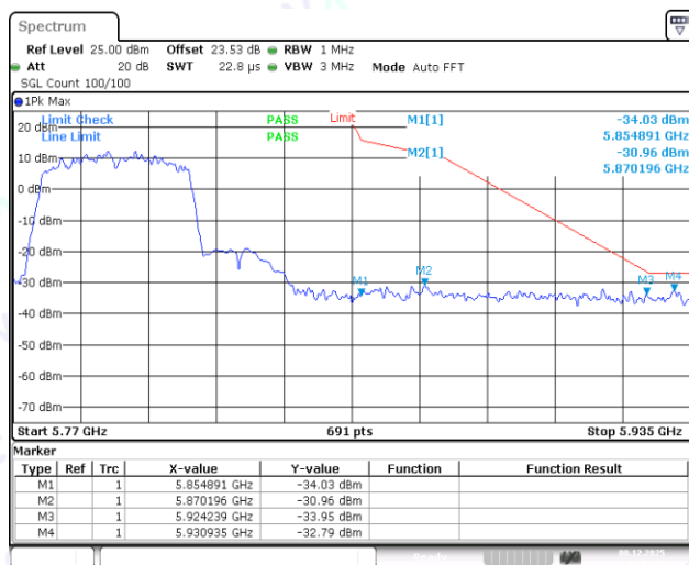
11N20SISO-Ant1-5825-PASS
