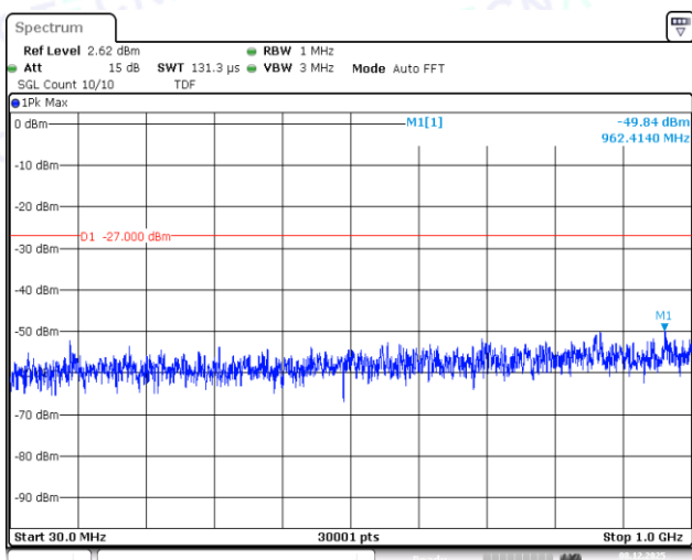
11AC20SISO-Ant1-5825-30~1000-PASS
