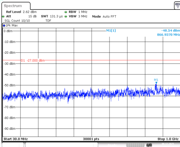
11N40SISO-Ant1-5190-30~1000-PASS
