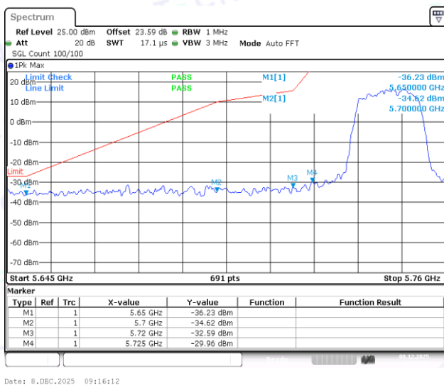
11A-Ant1-5745-PASS
