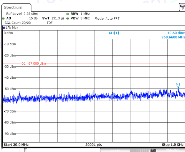
11N40SISO-Ant1-5230-30~1000-PASS
