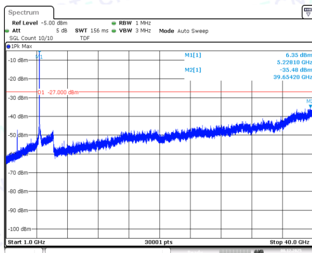
11AC40SISO-Ant1-5190-1000~40000-PASS
