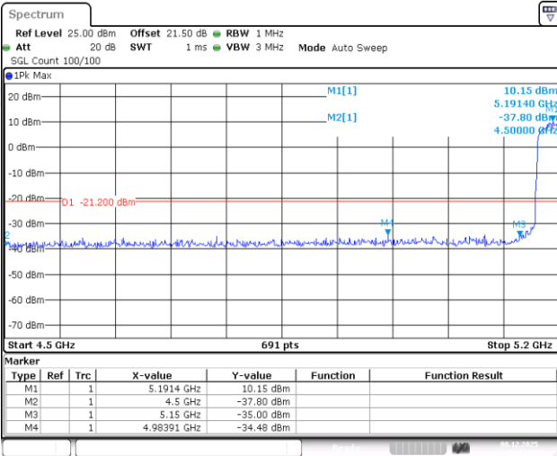
11AC40SISO-Ant1-5190-PASS
