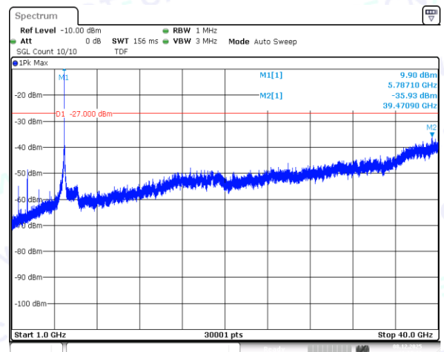
11AC20SISO-Ant1-5745-1000~40000-PASS
