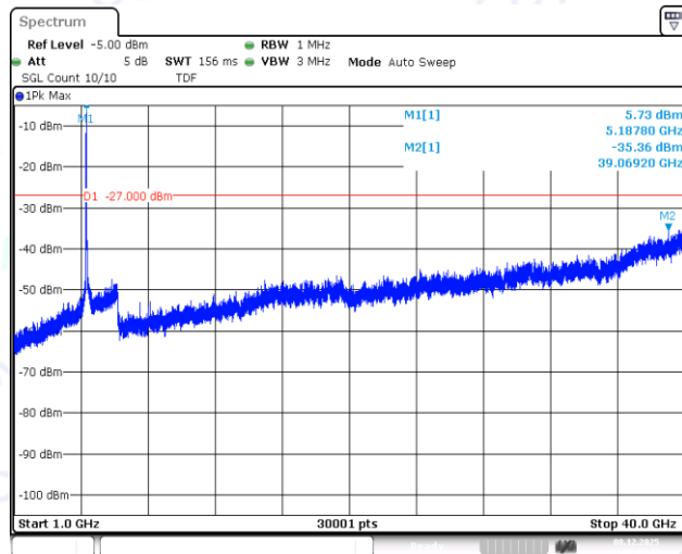
11N40SISO-Ant1-5190-1000~40000-PASS
