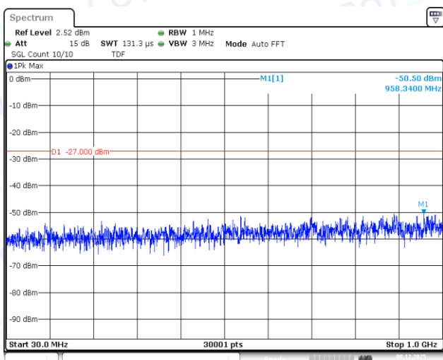
11AC40SISO-Ant1-5190-30~1000-PASS
