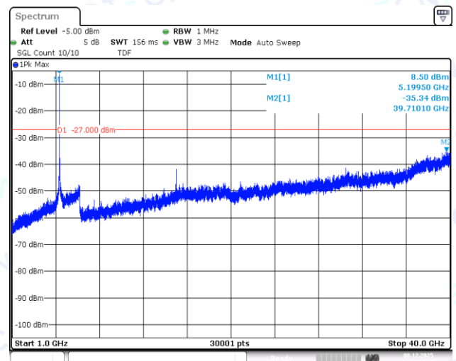
11AC20SISO-Ant1-5200-1000~40000-PASS
