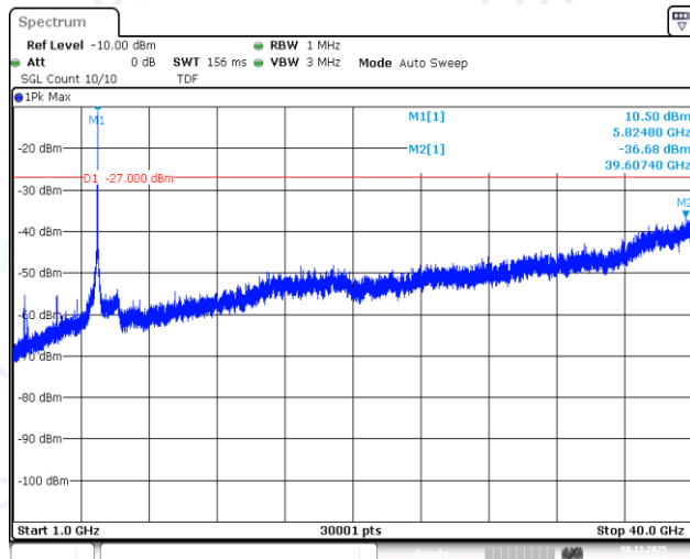
11AC20SISO-Ant1-5825-1000~40000-PASS
