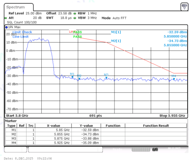
11A-Ant1-5825-PASS
