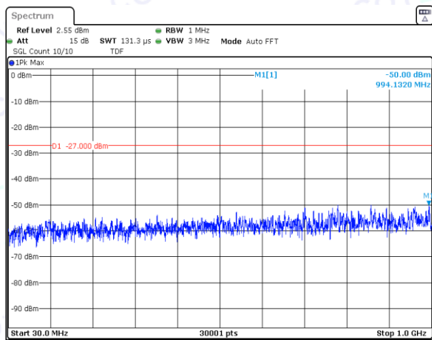
11A-Ant1-5180-30~1000-PASS
