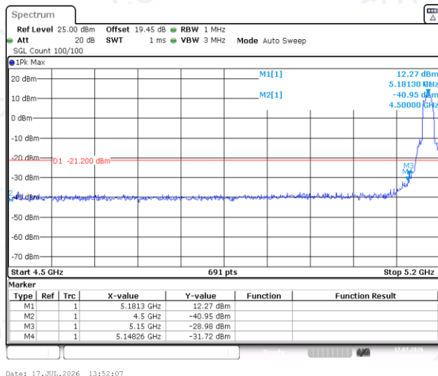
11A-Ant1-5180-PASS
