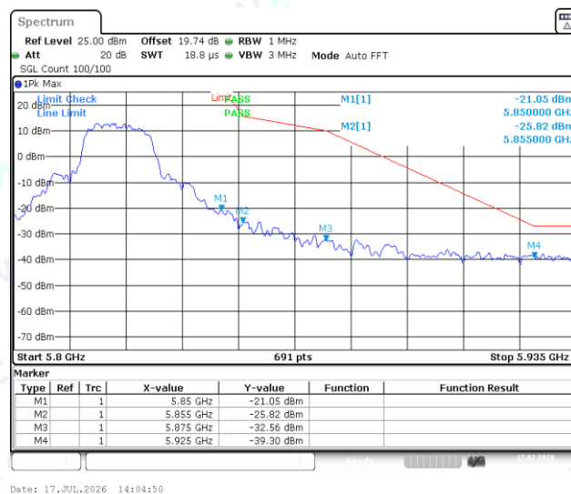
11A-Ant1-5825-PASS
