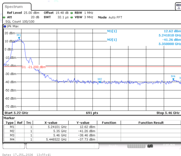
11A-Ant1-5240-PASS
