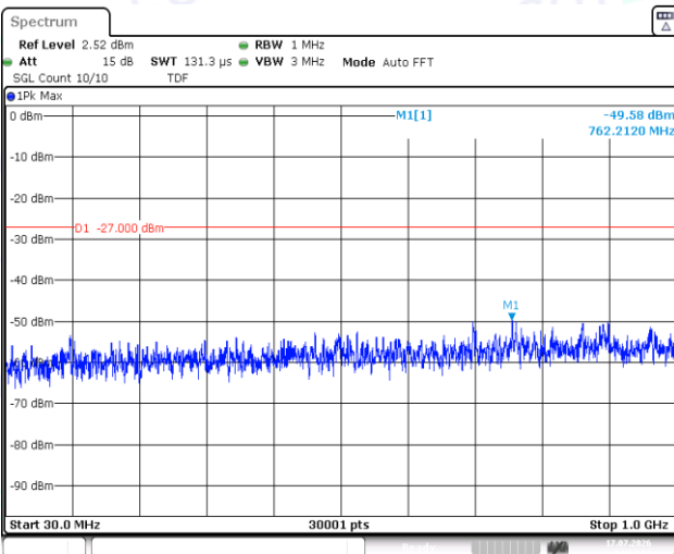
11N20SISO-Ant1-5200-30~1000-PASS
