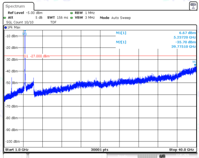
11AC40SISO-Ant1-5190-1000~40000-PASS
