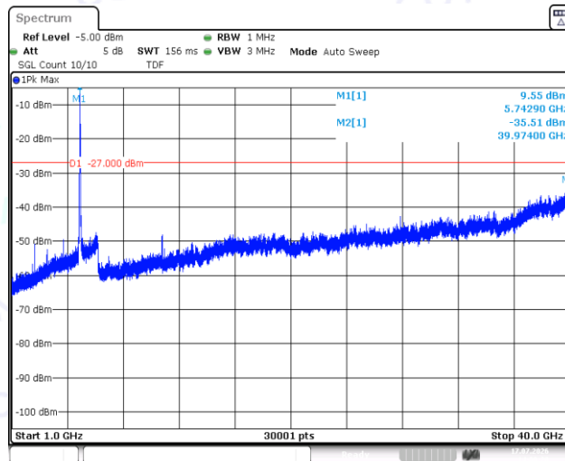
11A-Ant1-5745-1000~40000-PASS
