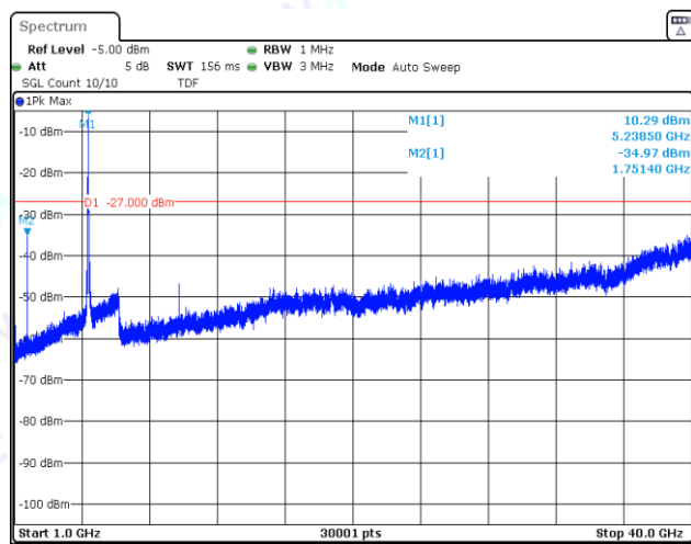
11A-Ant1-5200-1000~40000-PASS
