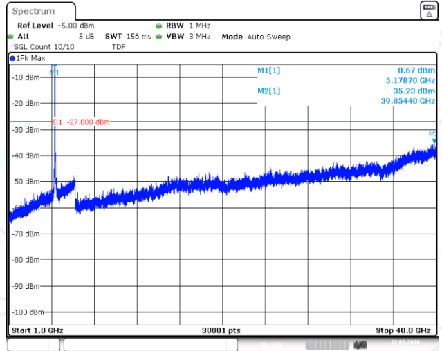
11N20SISO-Ant1-5180-1000~40000-PASS
