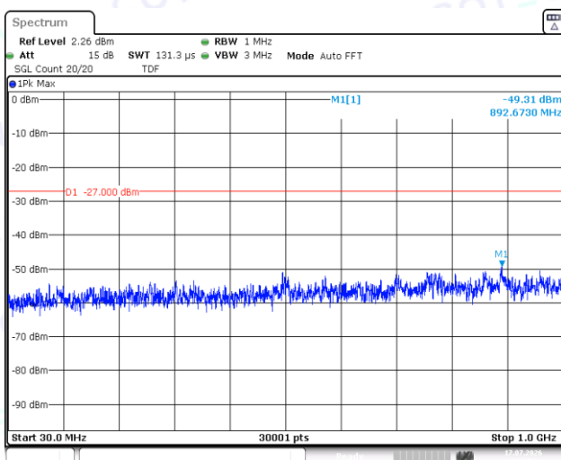
11A-Ant1-5785-30~1000-PASS
