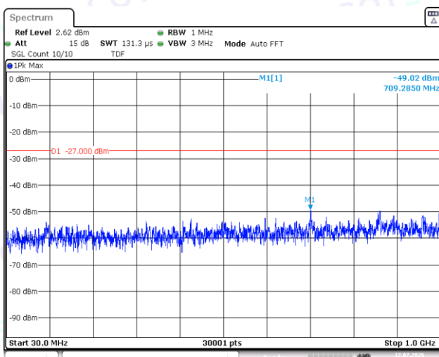
11AC20SISO-Ant1-5180-30~1000-PASS
