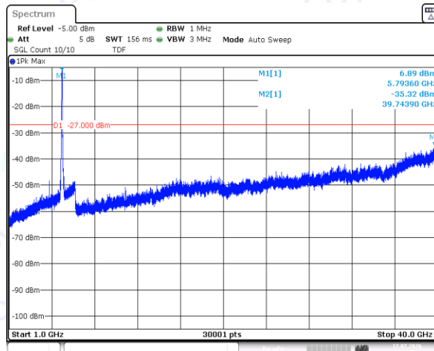
11N40SISO-Ant1-5795-1000~40000-PASS
