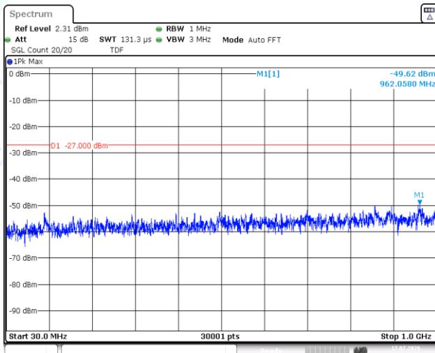
11N40SISO-Ant1-5795-30~1000-PASS
