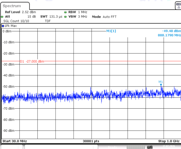
11AC40SISO-Ant1-5190-30~1000-PASS
