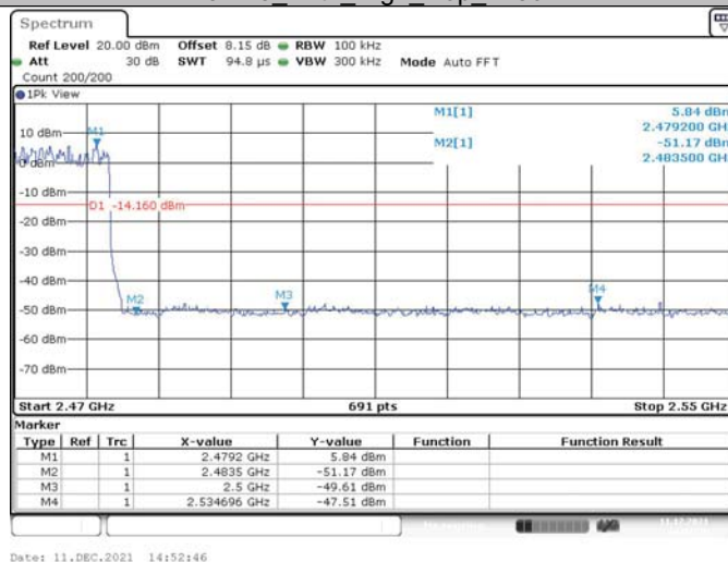
3DH5_Ant1_High_Hop_2480
