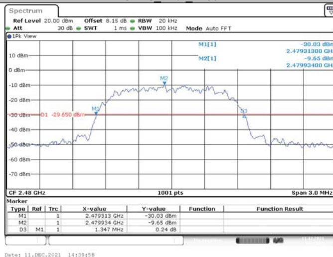
3DH5_Ant1_2480
