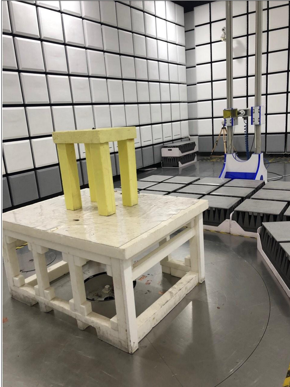
Frequency Range-Right Earphone < Above 1GHz >
