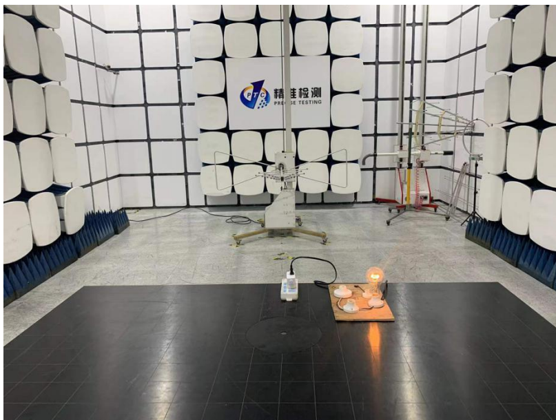
Radiated Emissions
