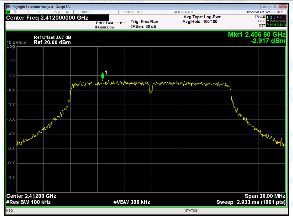
Tx. Spurious NVNT n(HT20) 2412MHz Ant1 Emission
