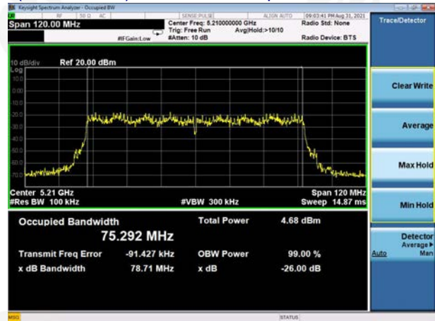
(802.11 ac80) 99%Bandwidth plot on channel 42
