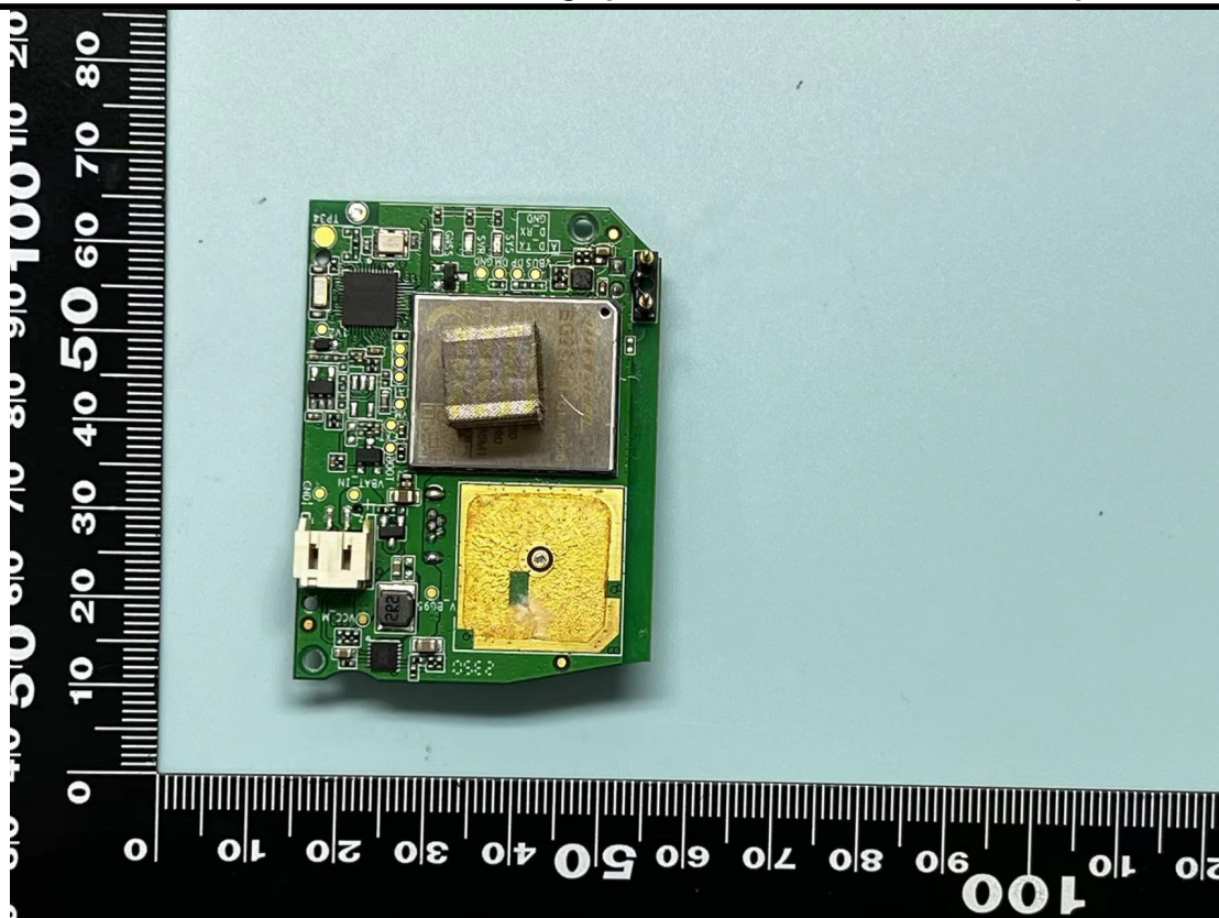
Top of PCBA
