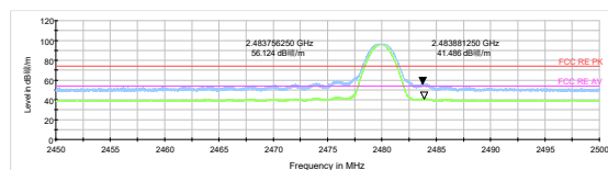
Bluetooth LE Channel 39 Peak+Average
