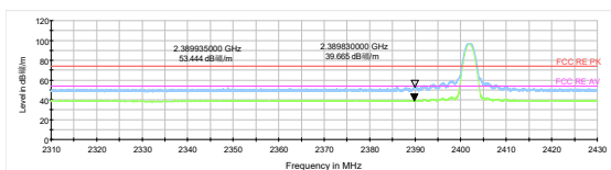
Bluetooth LE Channel 0 Peak+ Average
