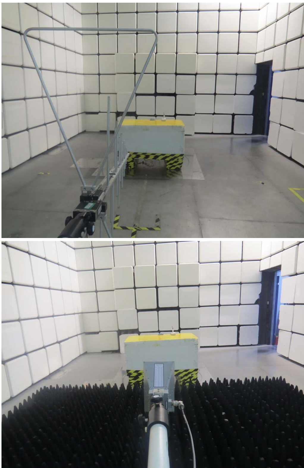
Picture 1: Radiated Emission Test Setup
