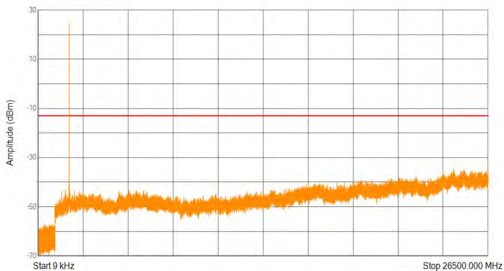
Band2 QAM16 BW=1.4MHz Channel=18607 RB Size=1 Position=#0 NB Index=0
