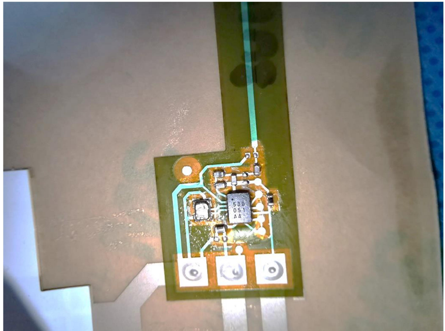
Solder Board-Component View
