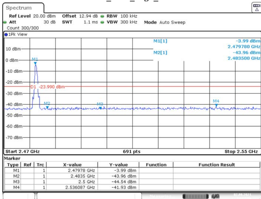
BLE_Ant1_High_2480
