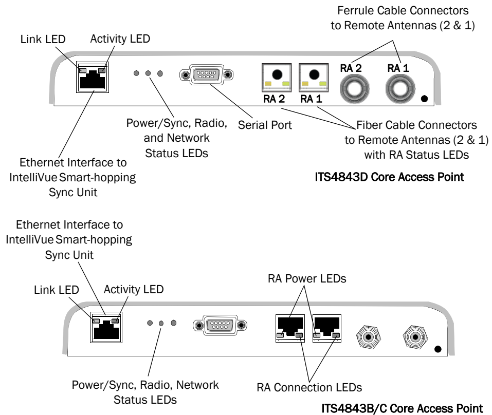
Figure 3-1: IntelliVue Smart-hopping Core Access Point LEDs
