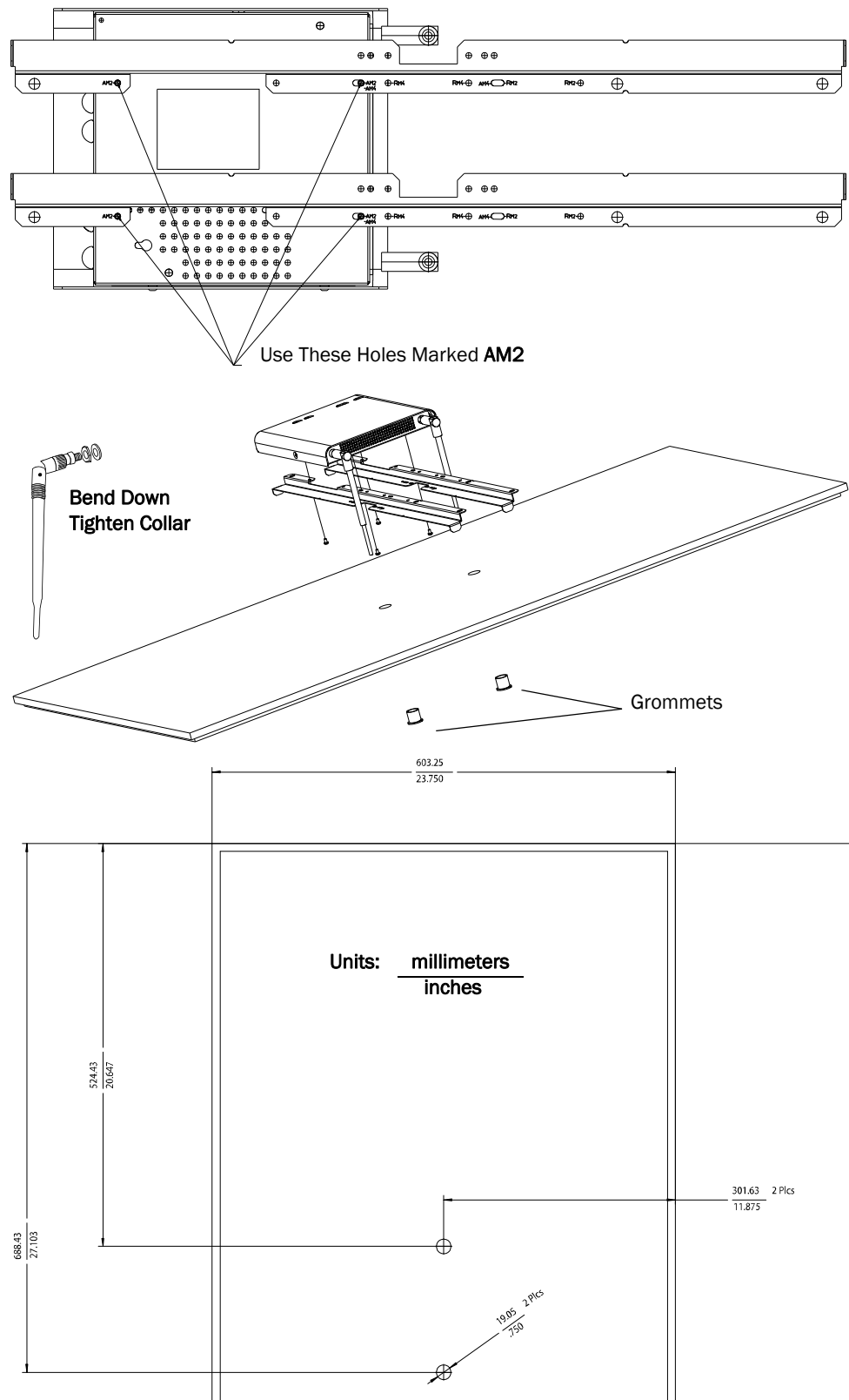
Figure 2-8: Possible Above the Ceiling Core AP Mounting Position
