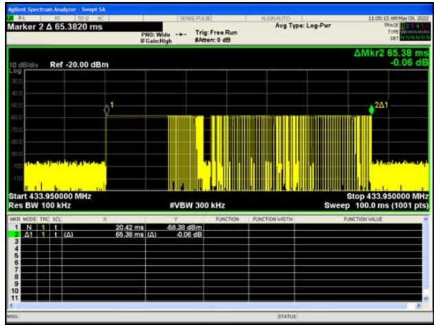
Pulse T on -1
