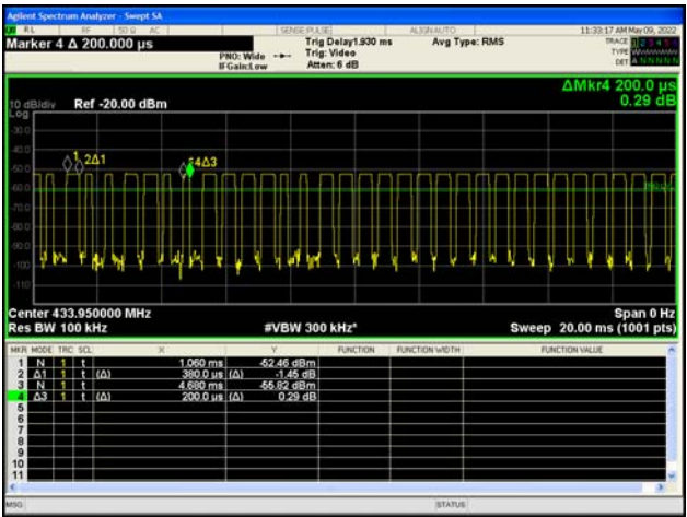
Pulse T on -2
