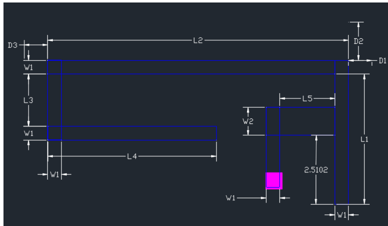
Figure 1: Antenna Dimensions
