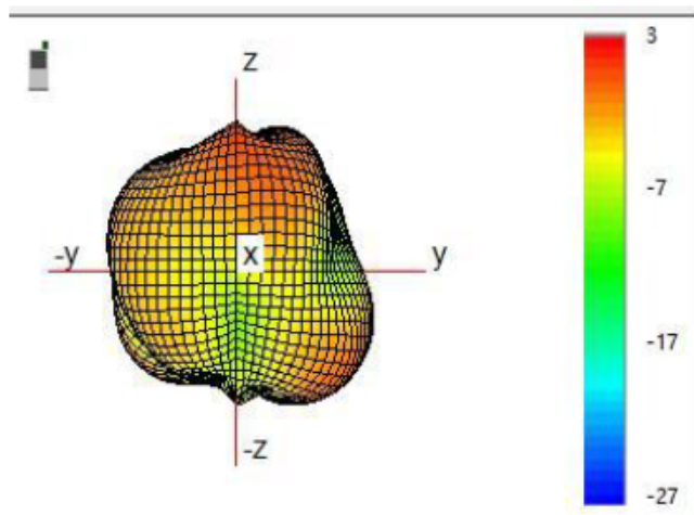
3D Gain Pattern @ 2450 MHz Unit: dBi
