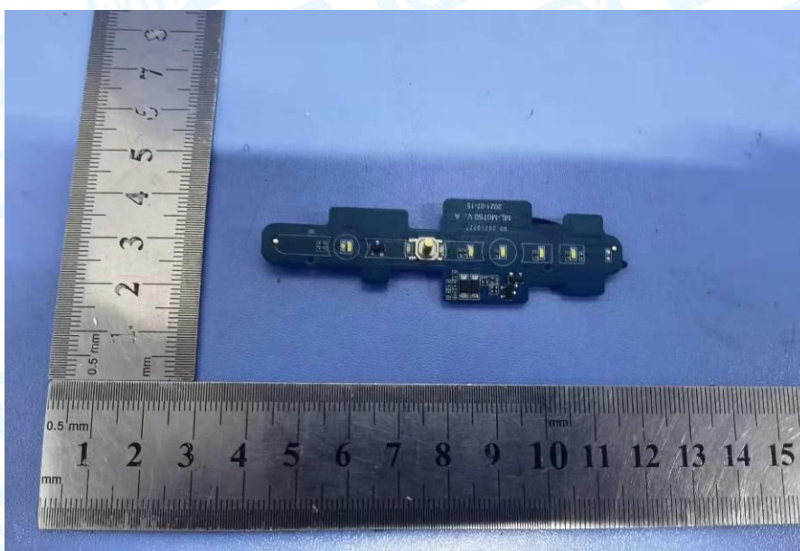
Photo 8 Internal of EUT
