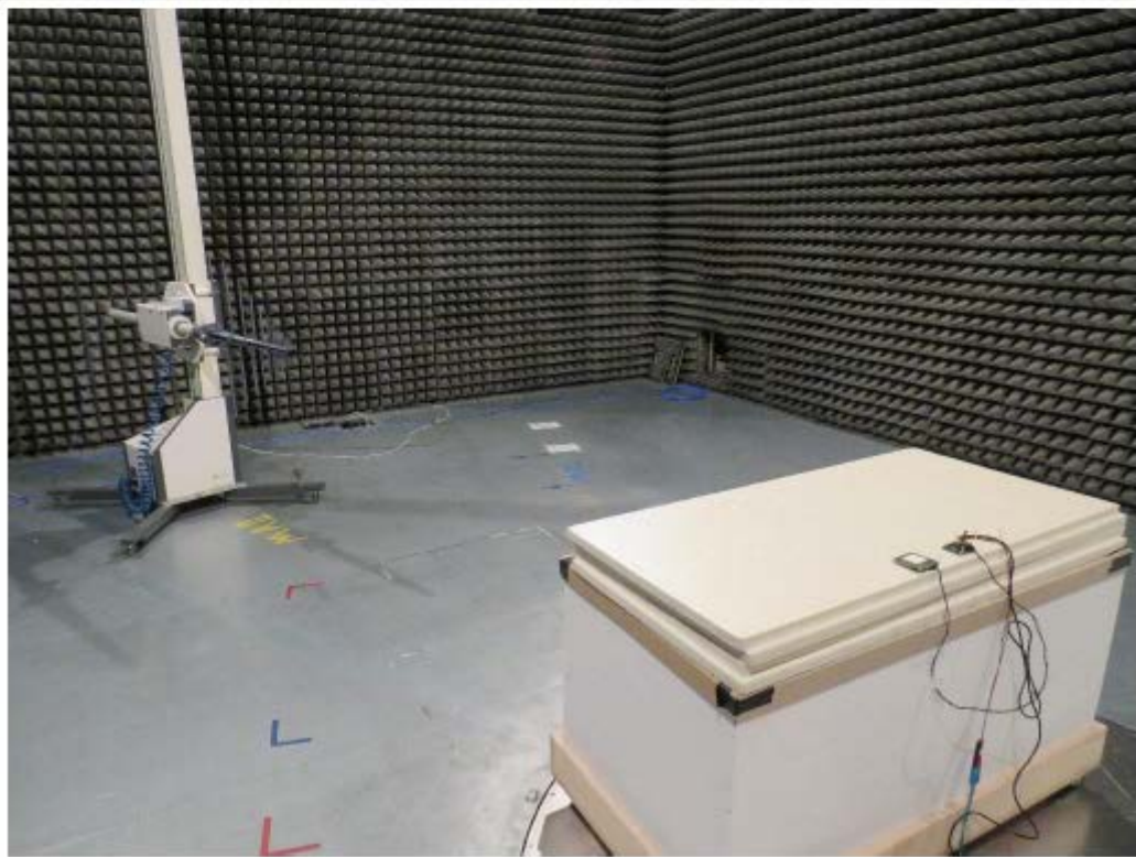
Setup 200 to 1000 MHz
