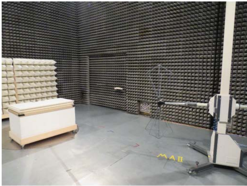
Setup 30 to 200 MHz
