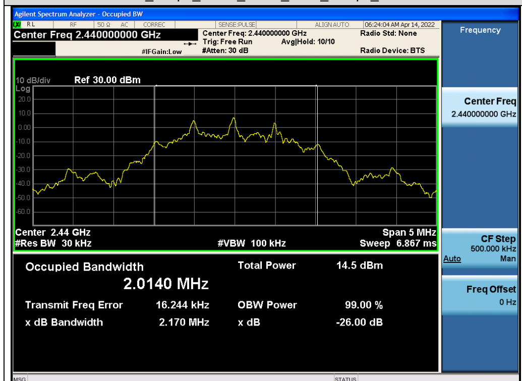
Test_Graph_LE2M_ANT1_2440_2Mbps_OBW
