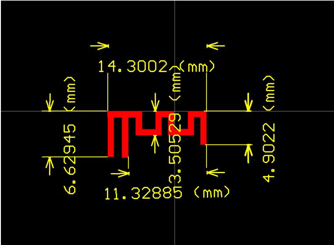
Antenna dimension drawing
