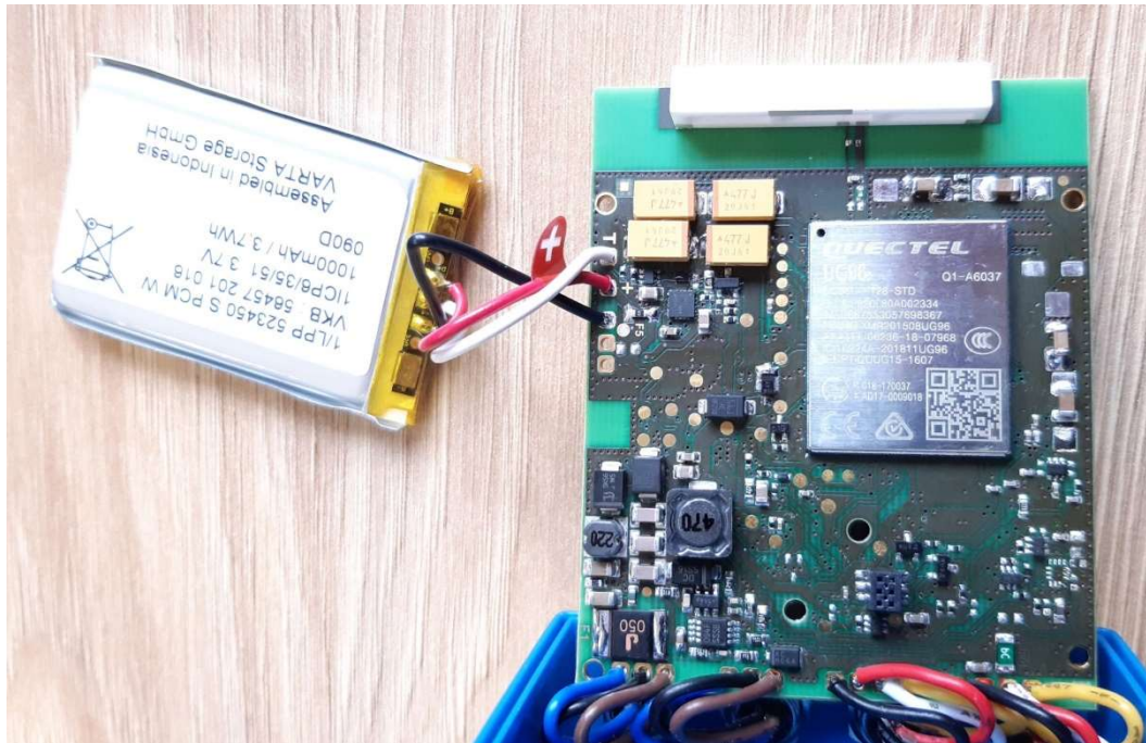
Main board - Front Top
