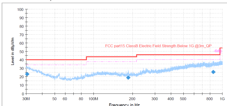
Figure 20: Spectral Diagrams, Radiated Emission, Mode D
