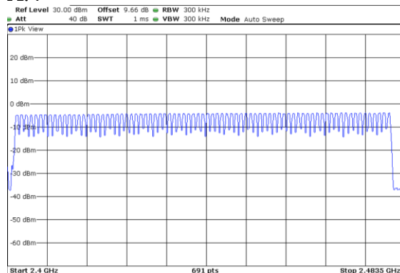
Figure 3: Number of hopping channels
