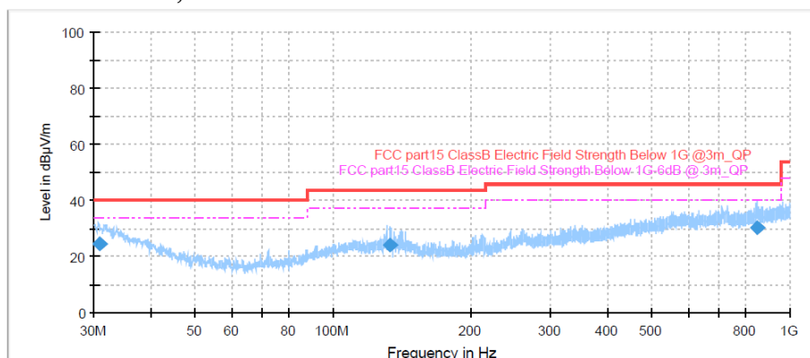
Figure 19: Spectral Diagrams, Radiated Emission, Mode C
