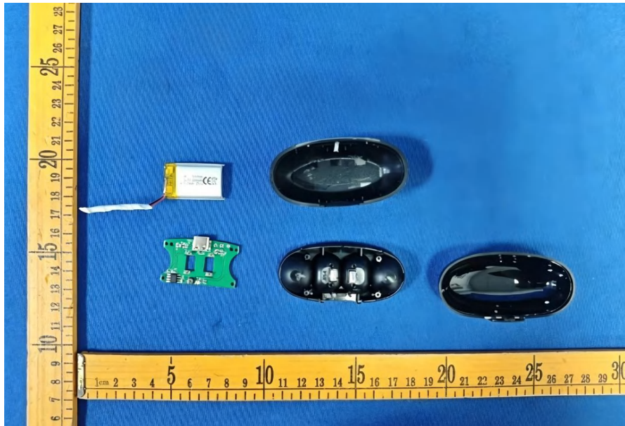
Charging case
