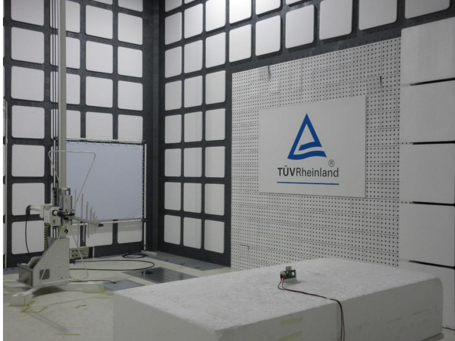
Photograph 3: Test Setup for Spurious Emissions (Back View 2, 3.3Vdc)
