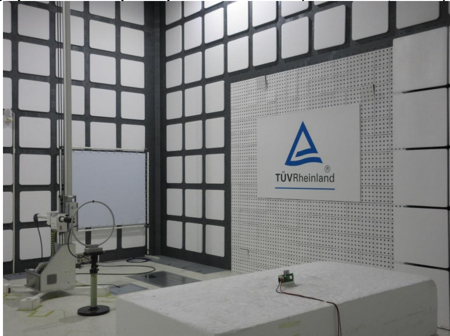
Photograph 2: Test Setup for Spurious Emissions (Back View 1, 3.3Vdc)
