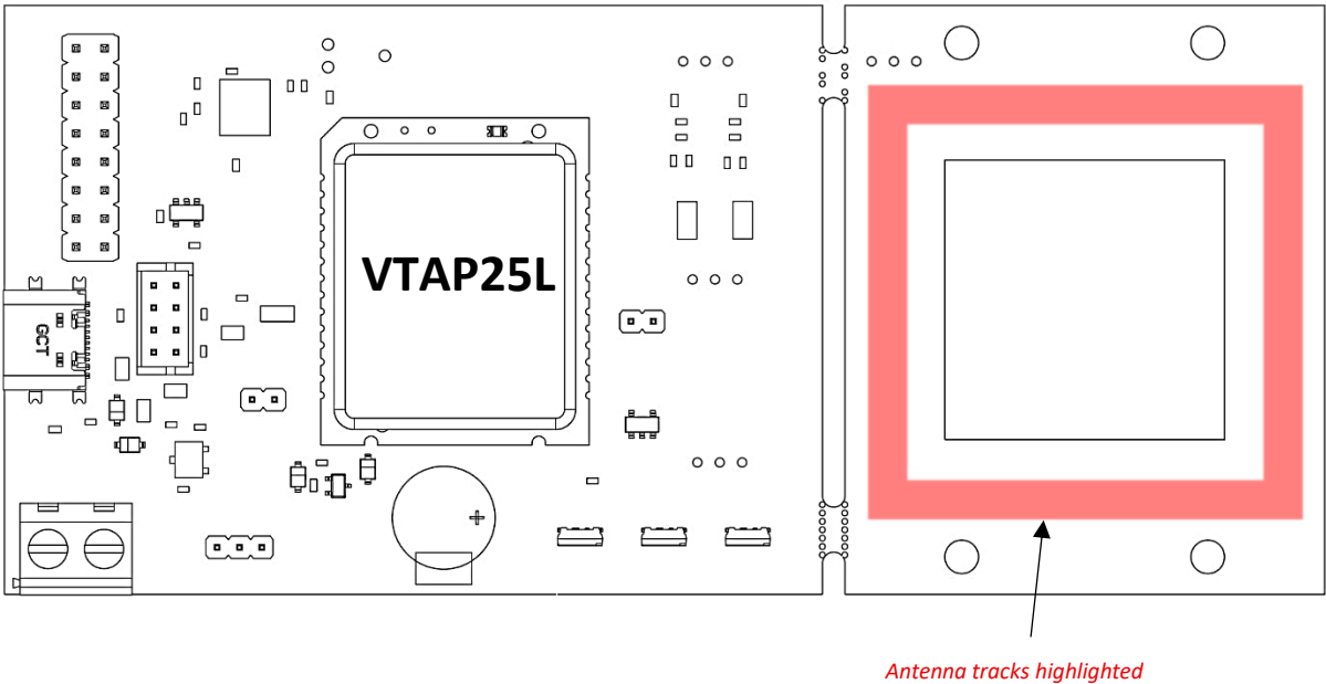
NFC Antenna Location
